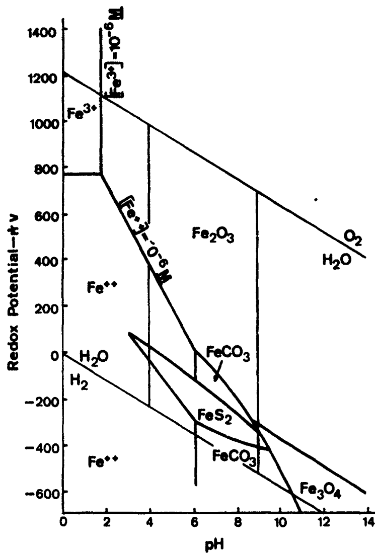
Figure 1. Redox Potential-pH Diagram for Simple Ions and Hydroxides of Iron at 25°C. 24 "From Introduction to Geochemistry by K. B. Krauskopf. Copyright 1967, McGraw-Hill Book Company. Used with permission of McGraw-Hill Book Company.
