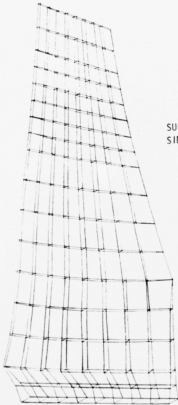
Figure 33. J101 B/A1 Blade, TAMP Model.
