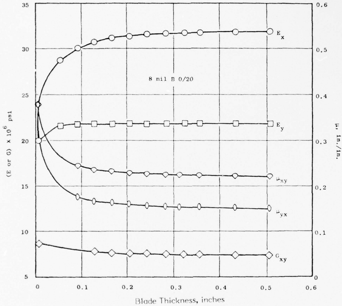
Figure 31. Influence of Nickel Plating on Elastic Properties of 0^0 , 20^0 B/Al at Various Blade Thicknesses.
