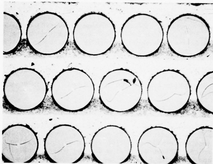
8 mil B-1000/2024 Hybrid Construction
