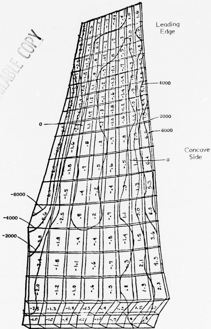
Figure 50. J101 B/A1 Blade TAMP Analysis, First Torsional, Radial Shear Stress ( \tau_{13} ).
