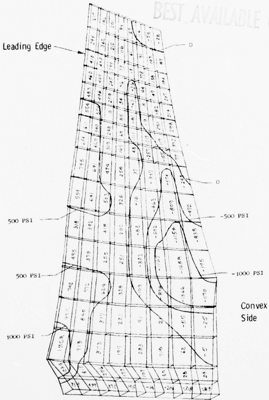
Figure 39. J101 B/A1 Blade TAMP Analysis, Chordwise Shear Stress, Convex ( \tau_{12} ).
