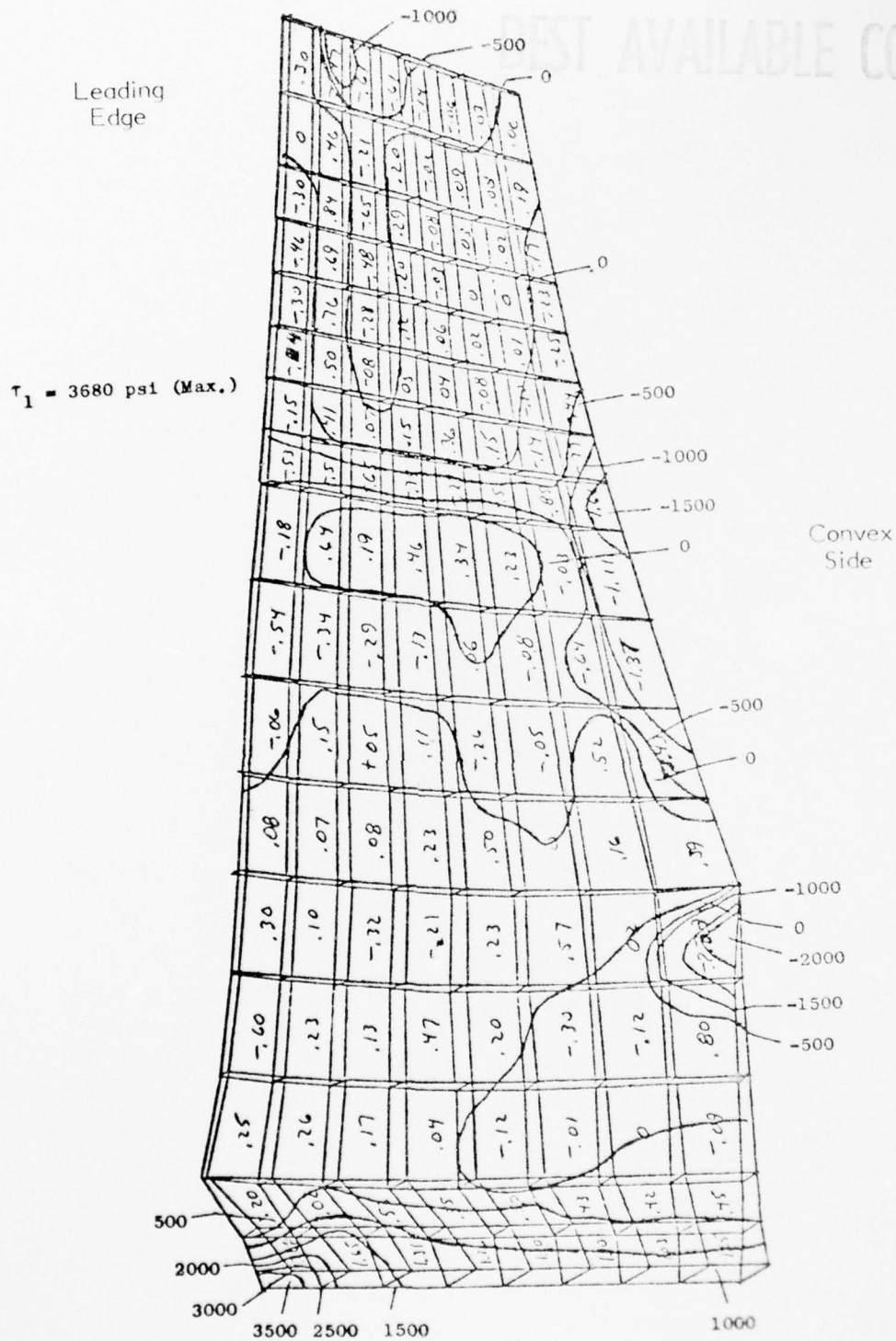
Figure 43. J101 B/A1 TAMP Analysis, Suction Side, Transverse Tensile Stress ( \tau_1 ).
