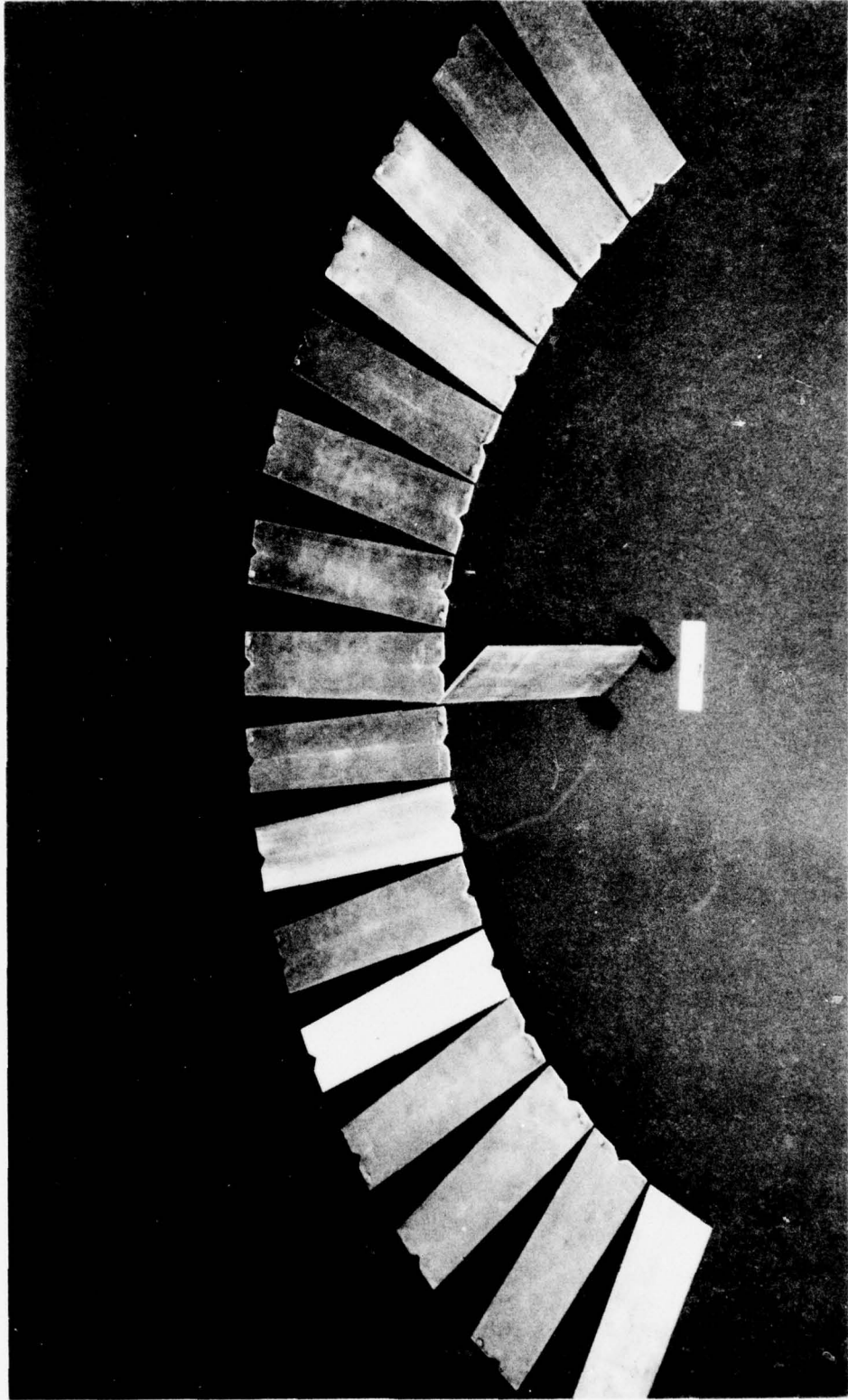
Figure 24. Air Bonded Blakelike Shape Specimens Produced for F0D Testing.
