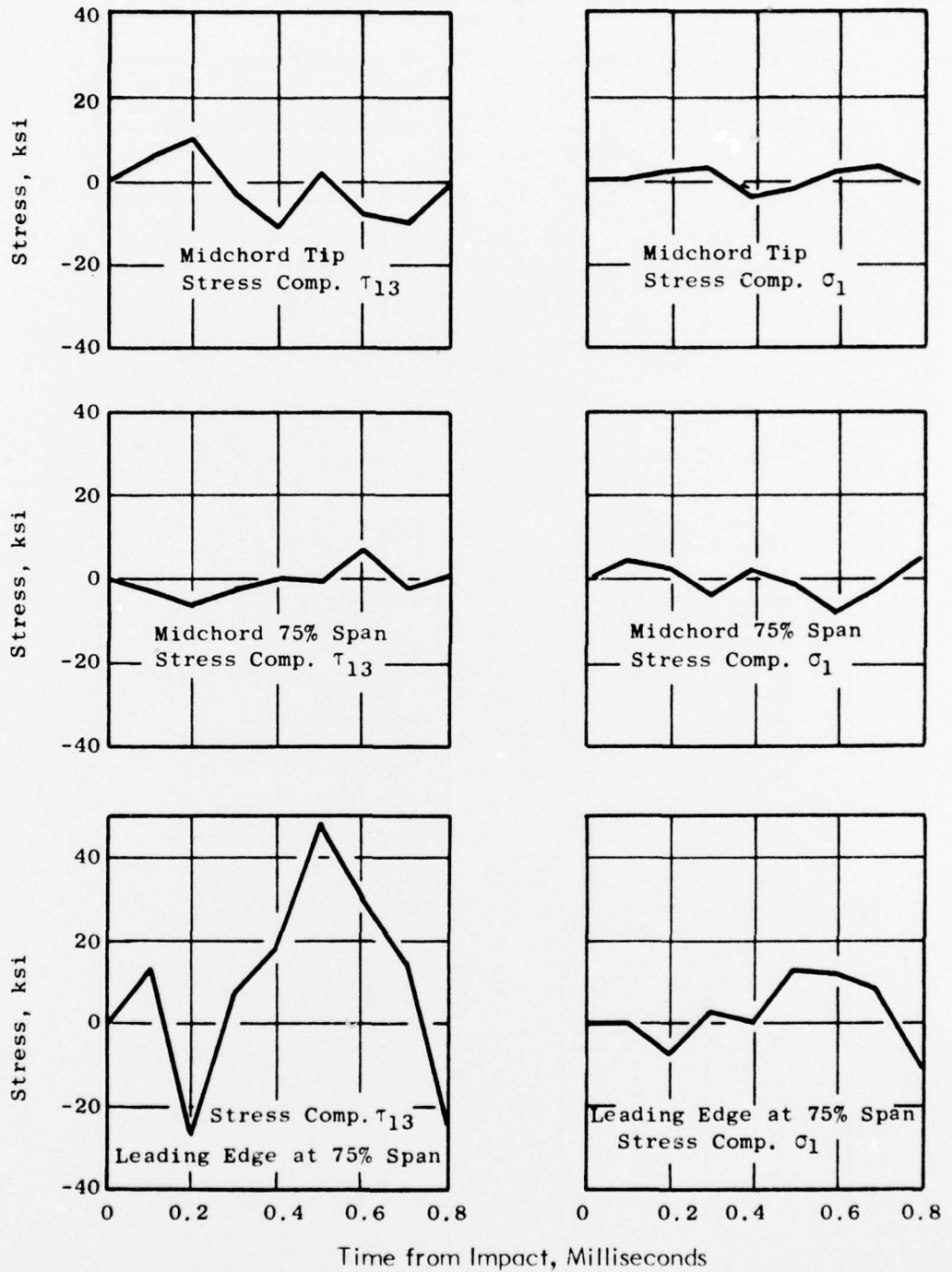
Figure 66. J101 B/A1 Blade Impact Results, 25 oz Bird.
