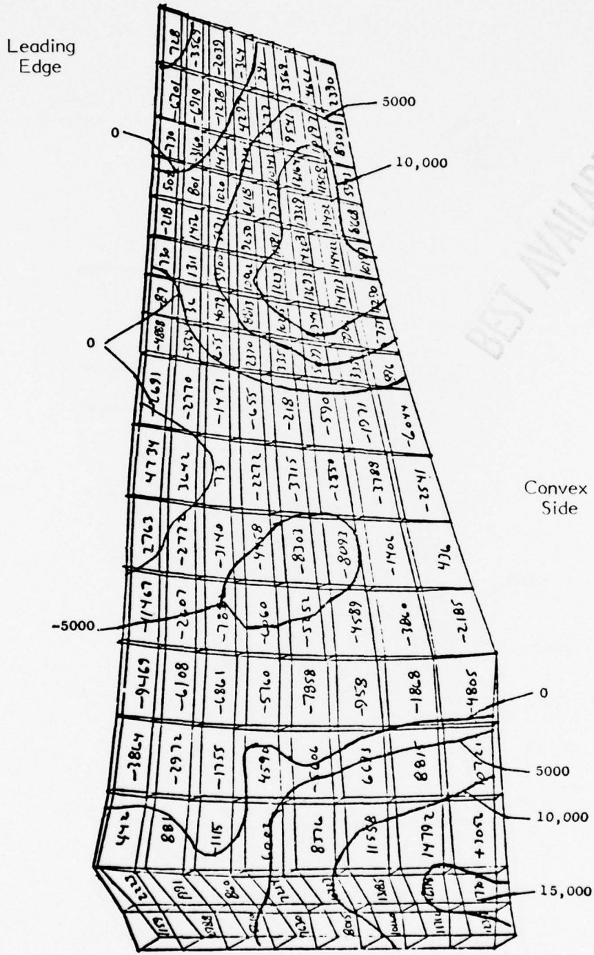
Figure 49. J101 B/A1 Blade TAMP Analysis, First Torsional, Radial Bending Stress ( \sigma_3 ).
