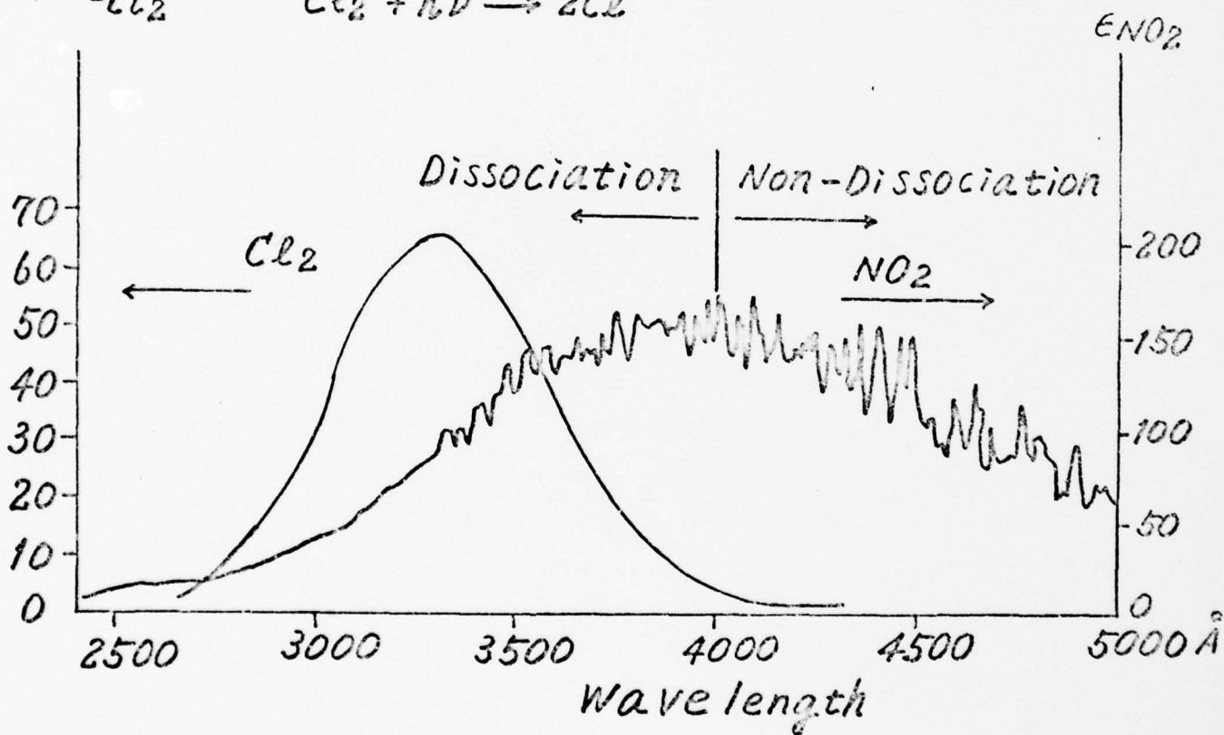
FIG. 5 ABSORPTION SPECTRA OF Cl_2 AND NO_2
