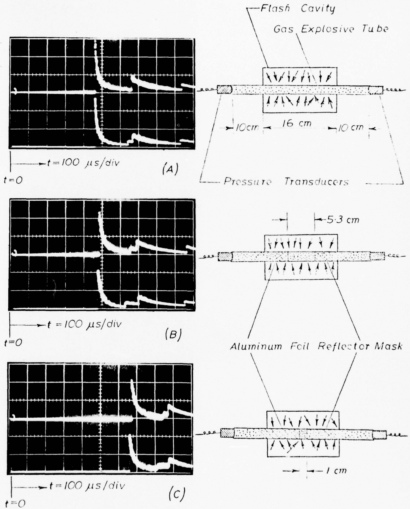
FIG. 10 Increase in Induction Time Due to Progressive Masking of the Irradiated Volume
