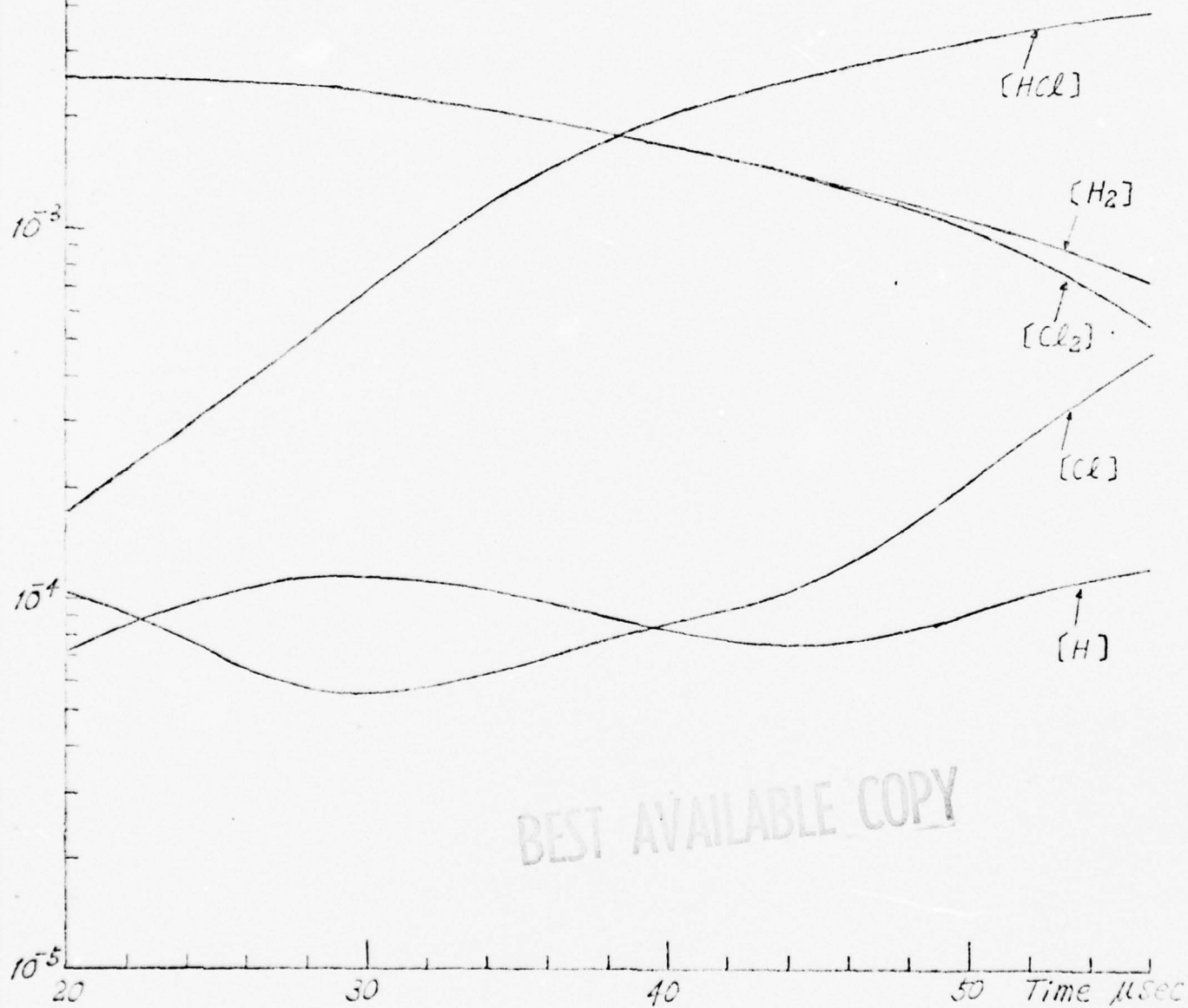
FIG. 14 PRODUCTION OF SPECIES BY PHOTOCHEMICAL INITIATION
