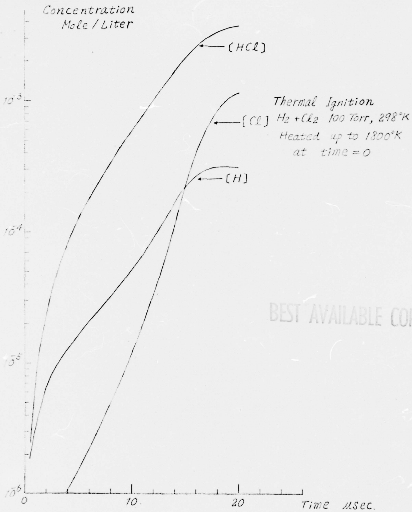
FIG. 26 PRODUCTION OF SPECIES BY THERMAL INITIATION
