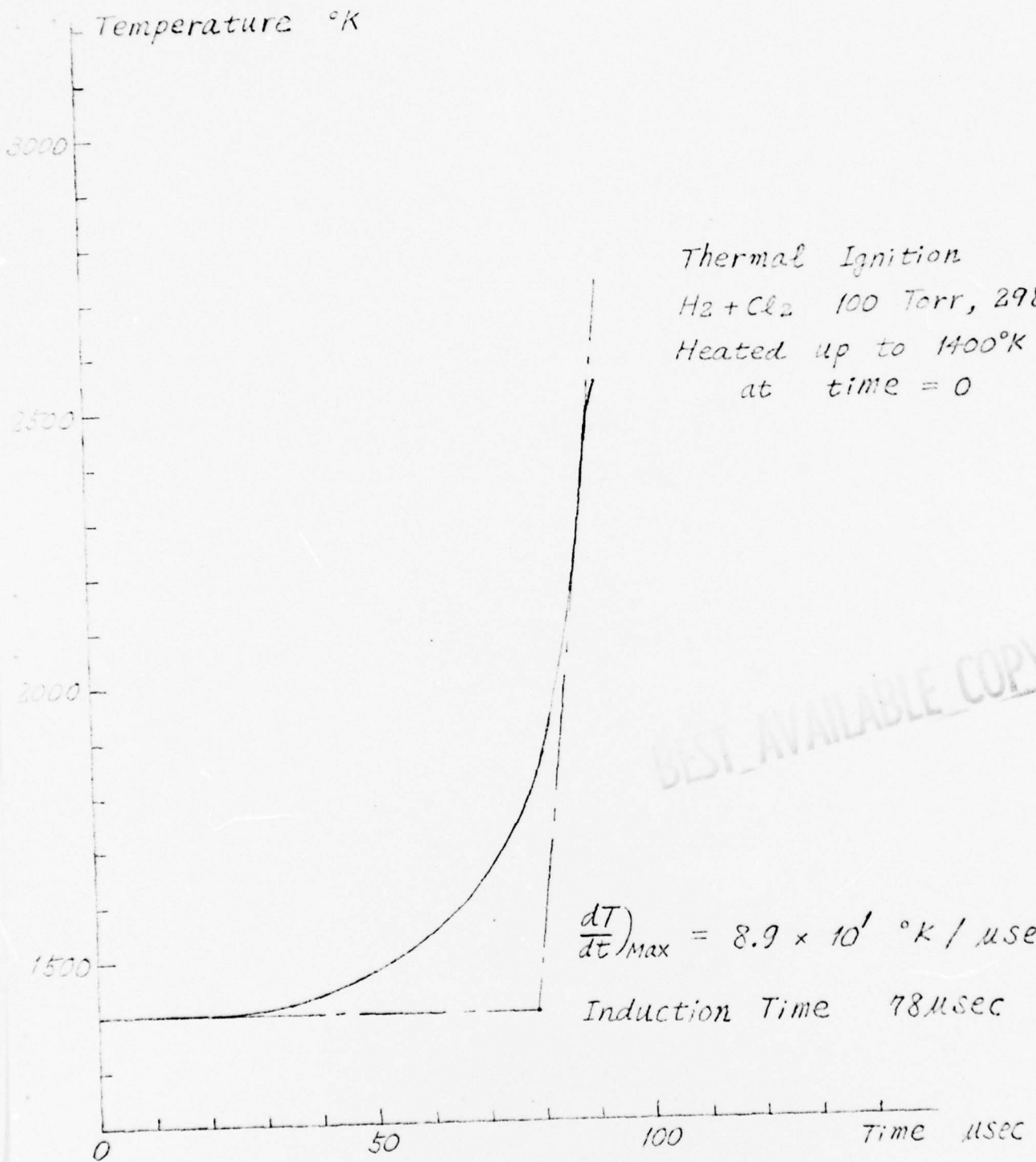
FIG. 27 TEMPERATURE-TIME PROFILES FOR THERMAL INITIATION
