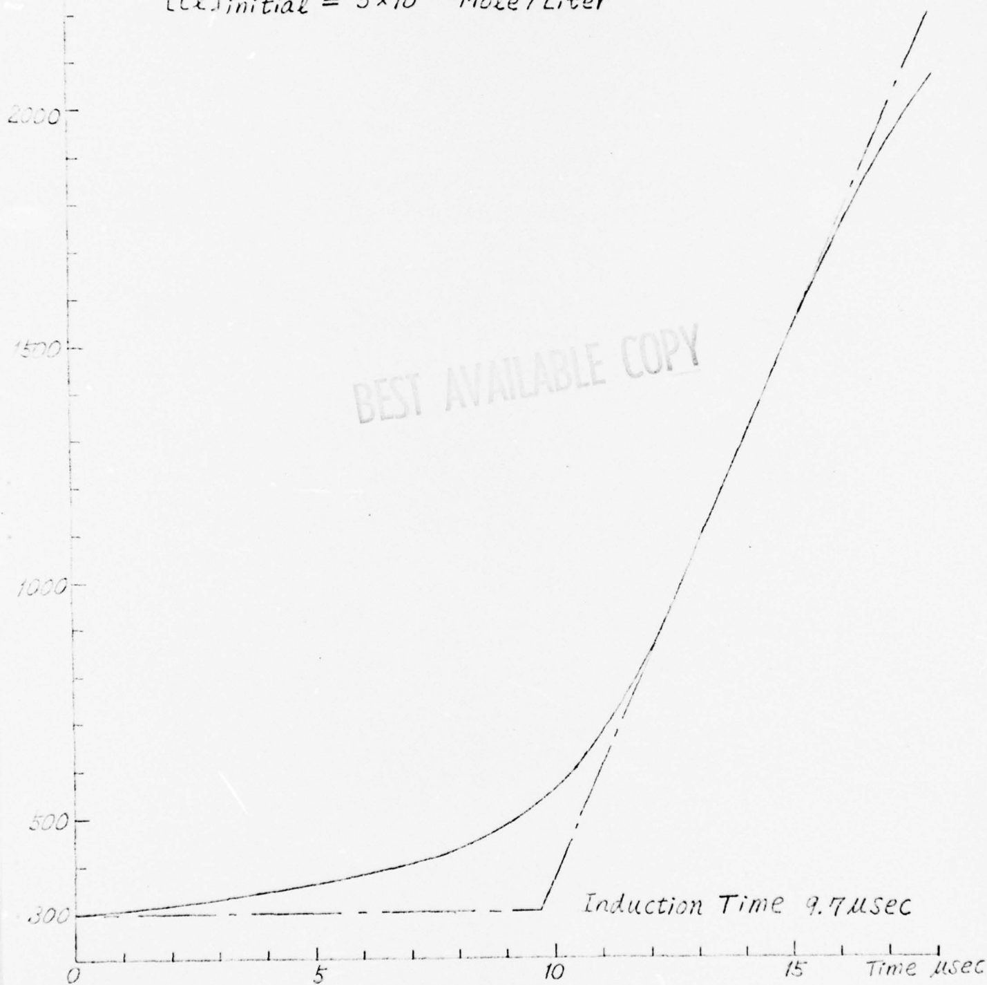
FIG. 21. TEMPERATURE - TIME PROFILES FOR PHOTOCHEMICAL INITIATION
