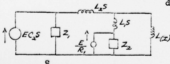
Fig.3-27 Reduction of Fig 3-26 To First Order Form of Fig. 3-20
