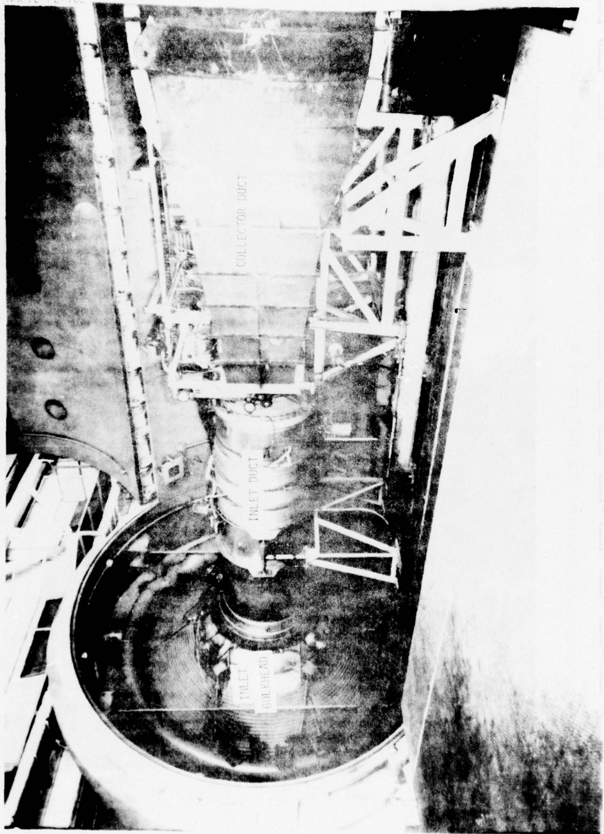
FIGURE 4: FOUR-POSTER V/STOL ENGINE INSTALLATION IN ALTITUDE CHAMBER 3E
