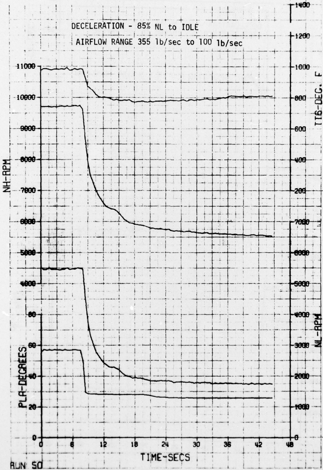
FIGURE 12: ENGINE DECELERATION AT SIMULATED SEA LEVEL STATIC CONDITIONS
