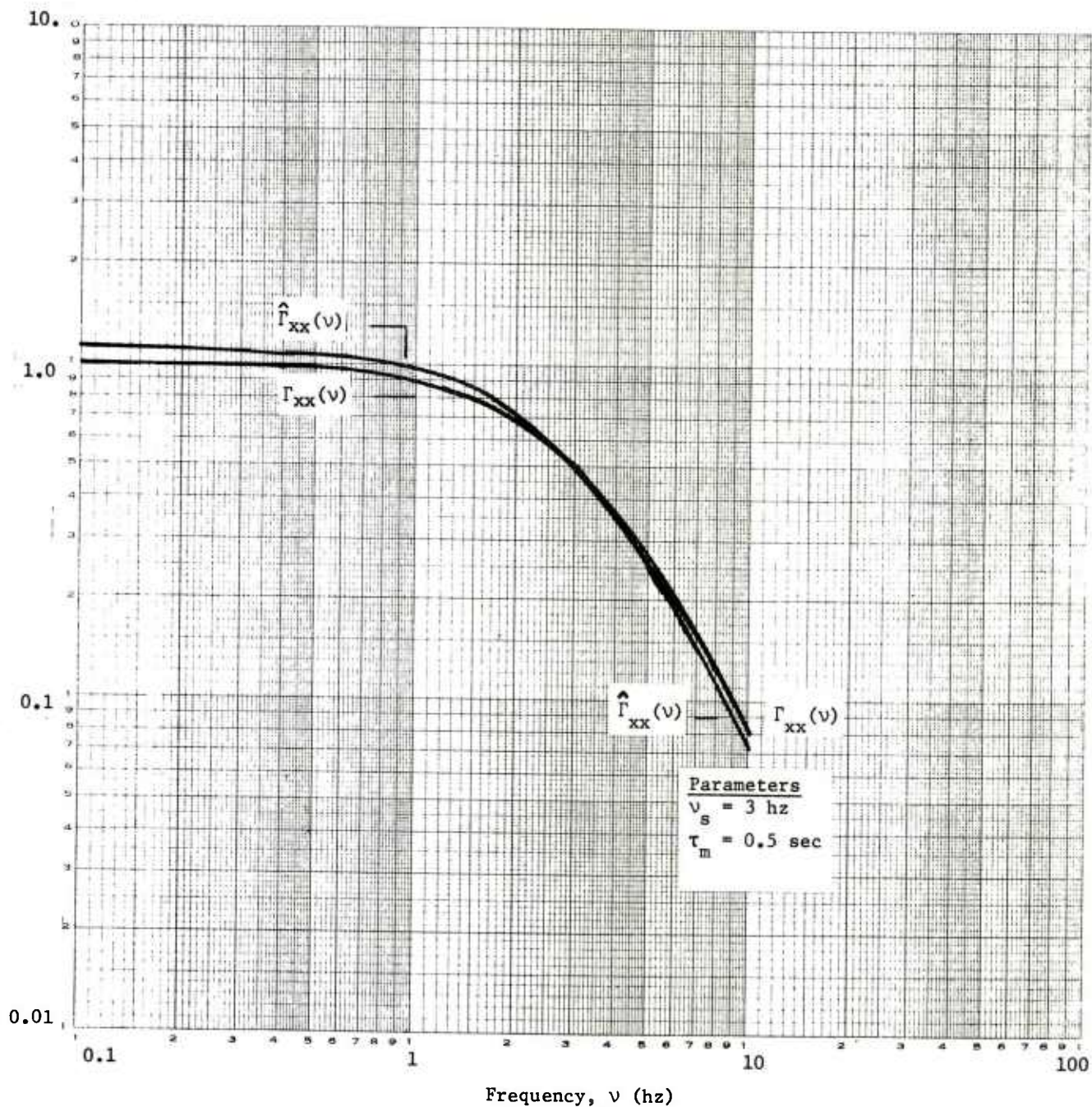
Figure 9. The Smoothed Autospectrum, \hat{\Gamma}_{xx}(\nu) , Due to a Bartlett Lag Window Applied to a First-Order Autocovariance With Associated Theoretical (Unsmoothed) Spectrum \Gamma_{xx}(\nu) (Parameters: \nu_s = 3 hz, \tau_m = 0.5 sec)
