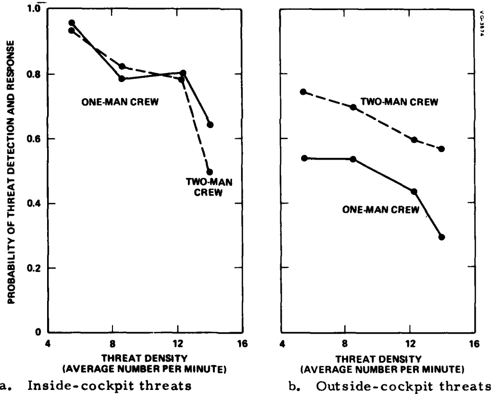
Figure 34. Comparison of inside- and outside-cockpit threats for one- and two-man crews and threat densities in the SAR target acquisition mission phase.
