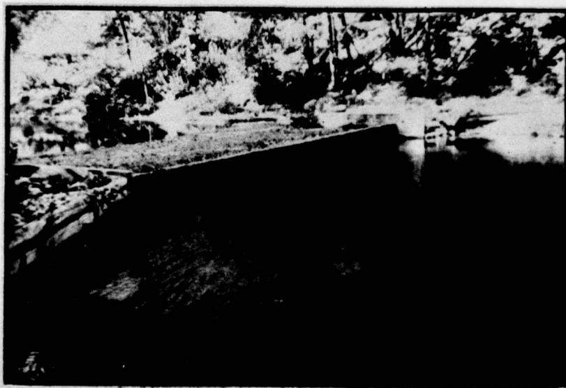
Photo No. 18 - A check dam on lower Oatka Creek to enhance the trout fishing. This reach of Oatka is a public fishing stream administrated by the Conservation Department, State of New York.
