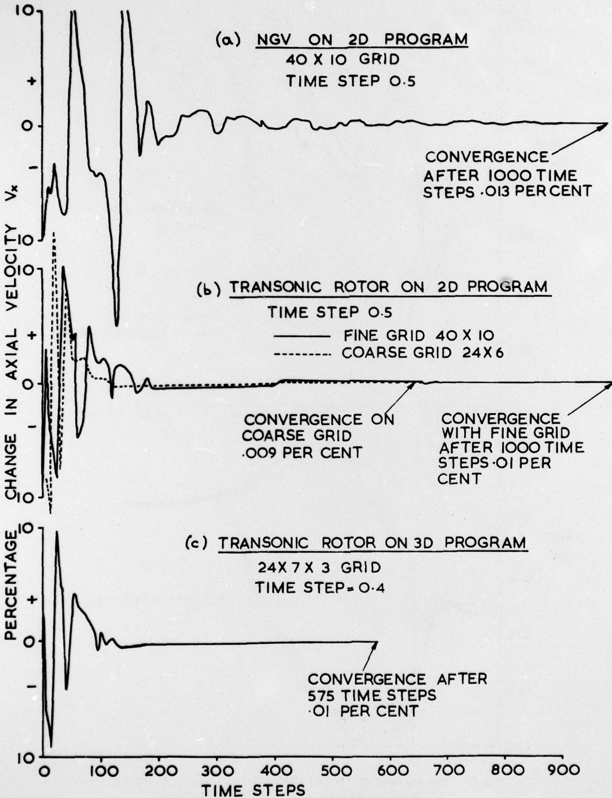
FIG. 4 RATE OF CONVERGENCE
