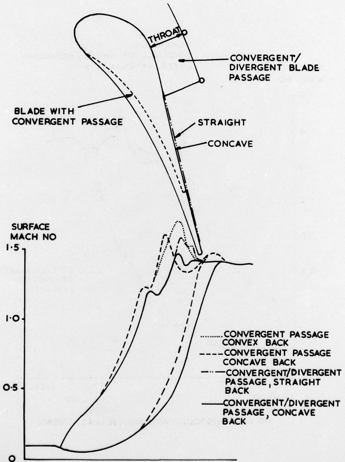
FIG. 14 NGV SURFACE MACH NUMBER DISTRIBUTIONS
