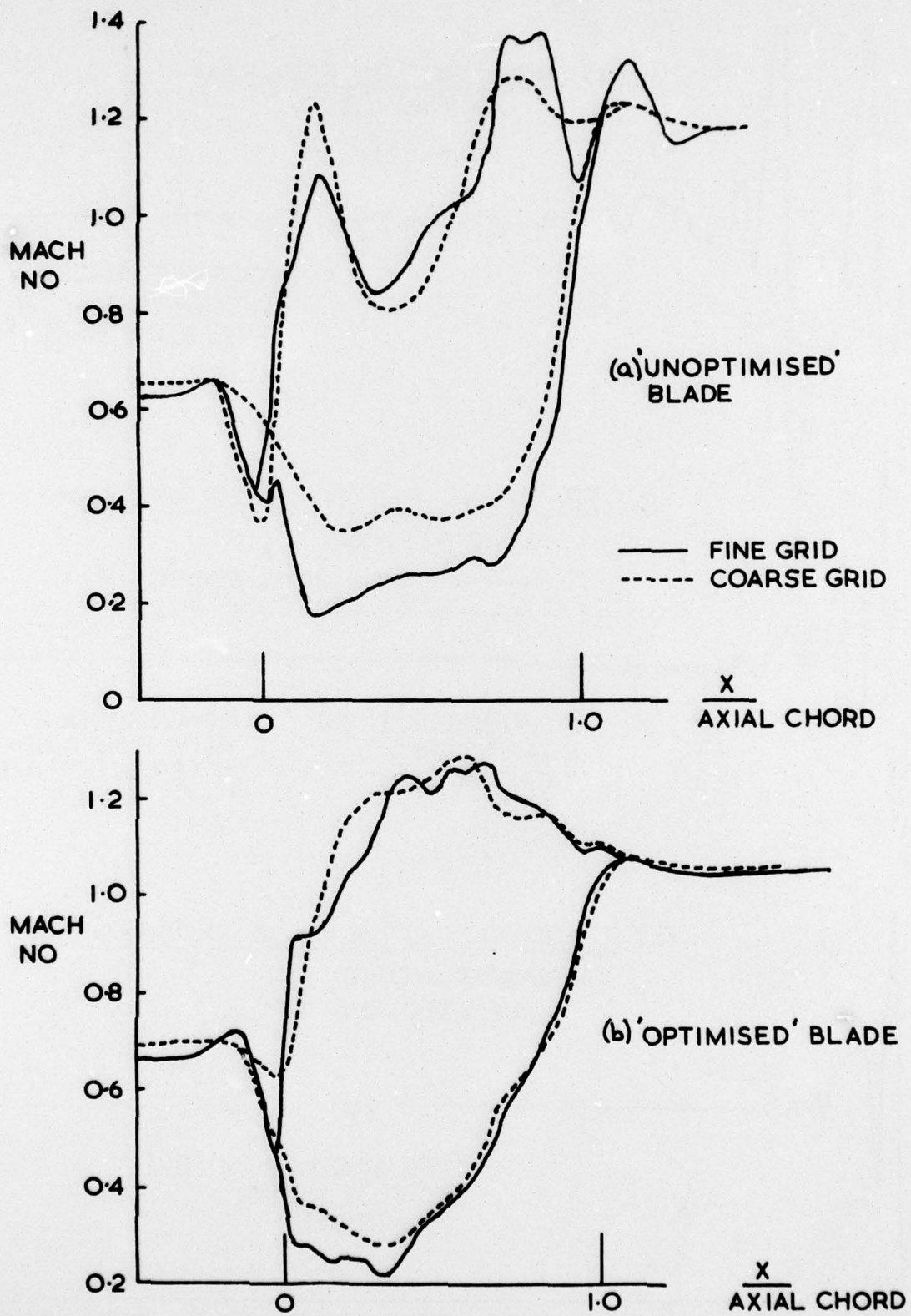
FIG. 3 TRANSONIC ROTOR BLADE SURFACE MACH NUMBER DISTRIBUTIONS FOR FINE AND COARSE GRIDS
