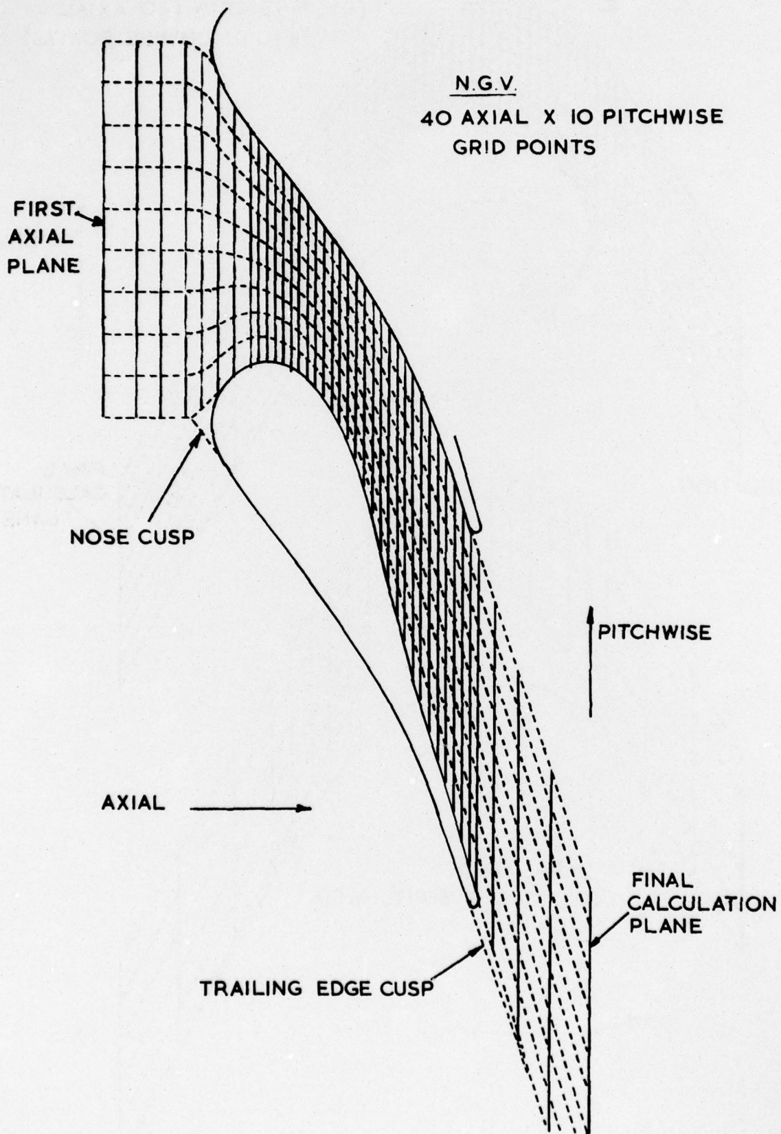
FIG. 1 TYPICAL GRID SPACING FOR A TRANSONIC NGV
