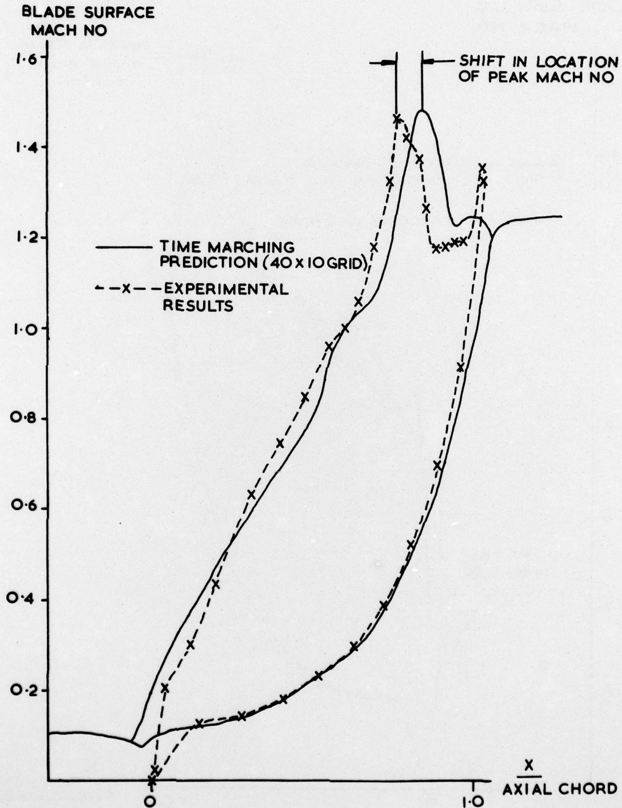
FIG. 7 TRANSONIC NGV IN A 2D CASCADE AT ZERO INCIDENCE
