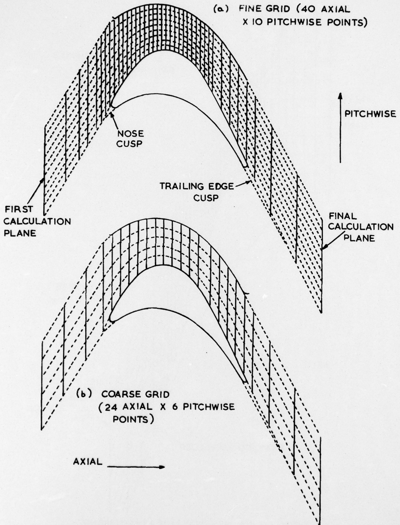
FIG. 2 TYPICAL GRID SPACING ON A TRANSONIC ROTOR BLADE
