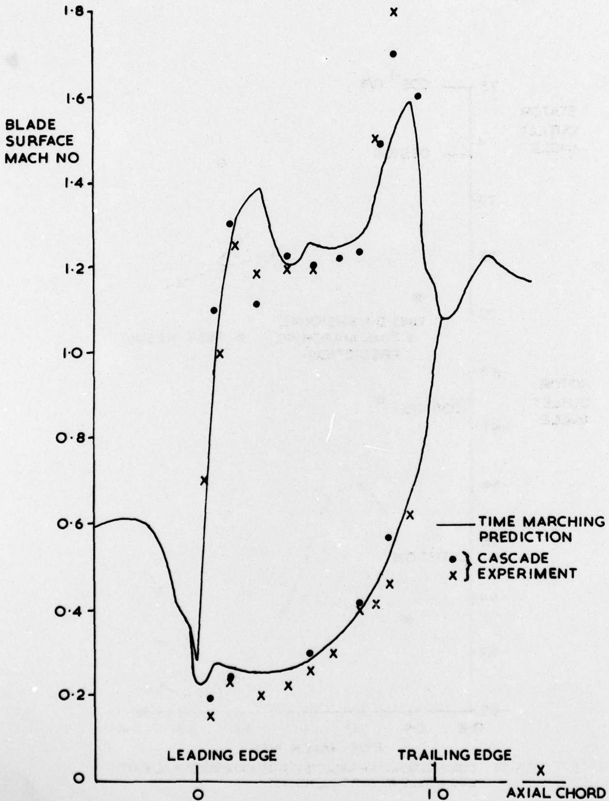
FIG. 12 TRANSONIC ROTOR BLADE CASCADE WITH WALL FLARE AT ZERO INCIDENCE
