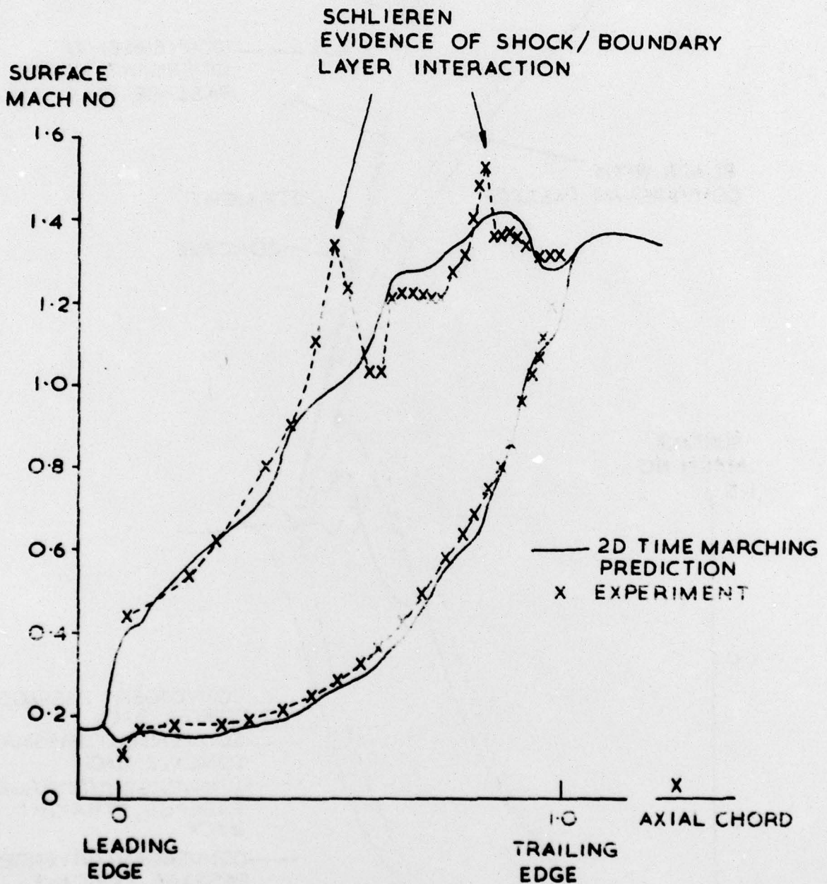
FIG. 13 CONVERGENT/DIVERGENT NGV IN A 2D CASCADE
