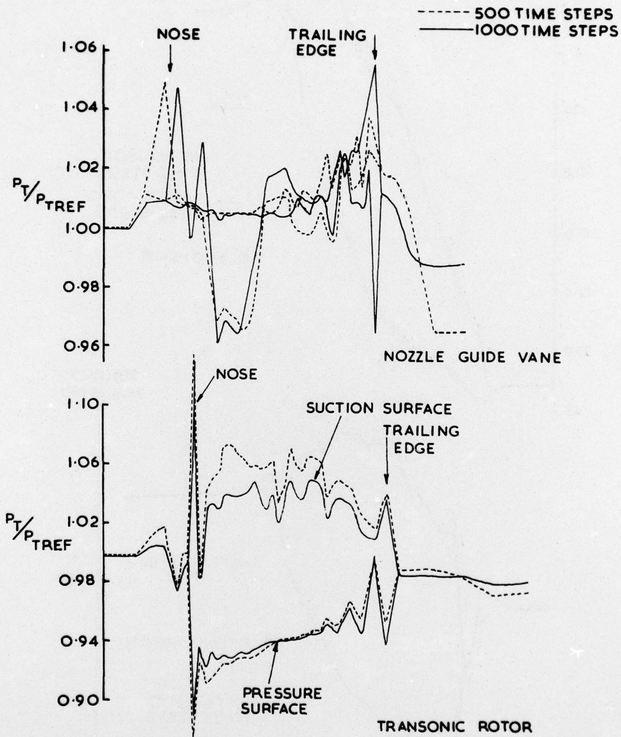
FIG. 6 TOTAL PRESSURE VARIATION IN THE BLADE CHANNEL - 2D SOLUTION 40 x 10 GRID
