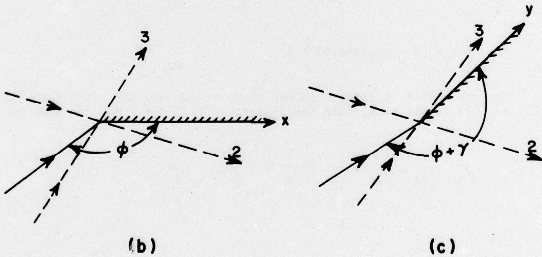
Figure 3. Wedge reflection geometry.
