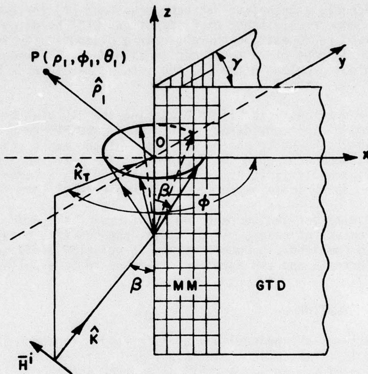
Figure 1. Wedge diffraction geometry used in MM-GTD solution.
