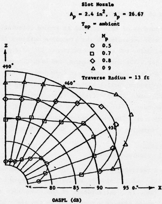
Figure 4.1. OASPL Directivities in the Flyover Plane of the Primary Slot Nozzle.
