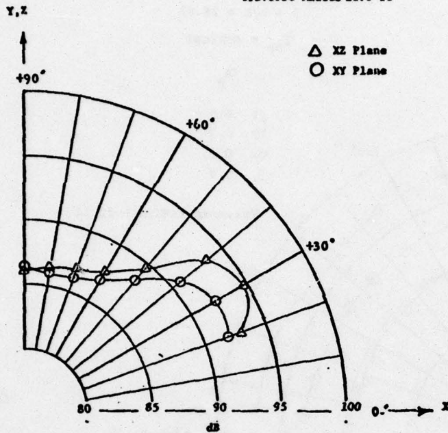
Figure 4.5a. Comparison of OASPL Directivity in XY and XZ Planes for Slot Nozzle of Aspect Ratio 27.0. (Ref. 13).
