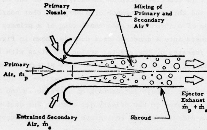
Figure 1.1. Configuration Sketch of Shrouded Nozzle.
