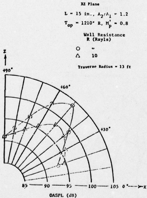
Figure 4.51. OASPL Directivity in XZ Plane of 15 Inch Shrouded Hot Jets with Hard Wall and Lined Shrouds.
