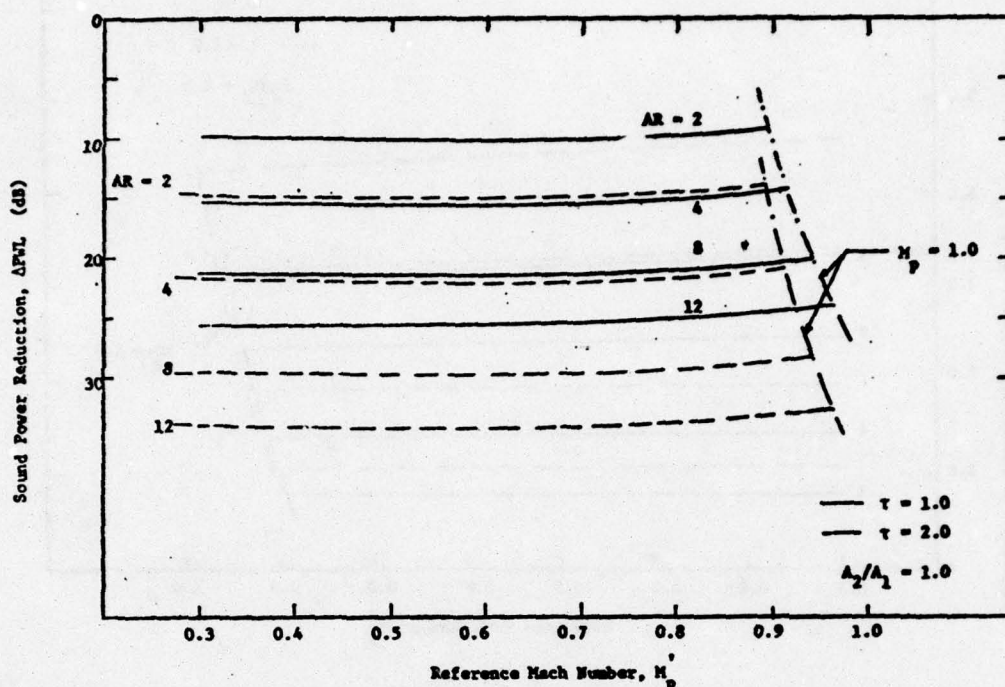
Figure 3.5. Sound Power Reduction, \Delta PWL as a Function of Reference Mach Number M_p^v for Constant Area Shrouded Nozzle.
