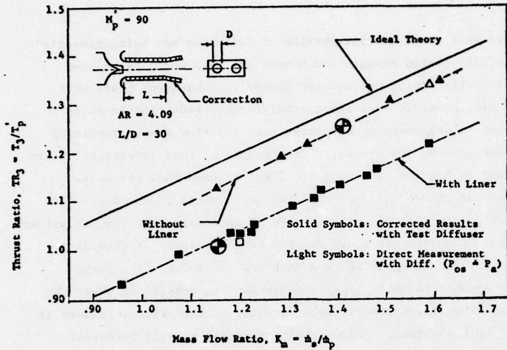
Figure 1.3. Summary of Thrust Results from Reference 1.
