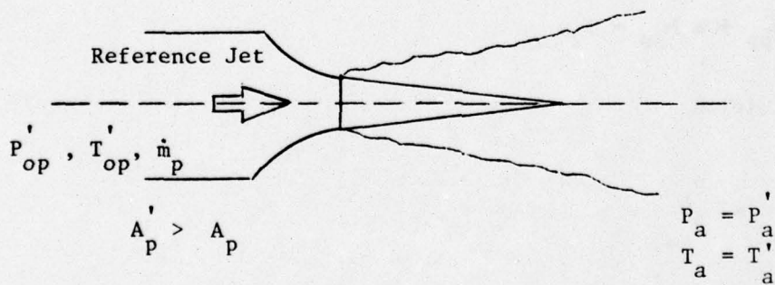
Figure 3.2. Reference Nozzle.
