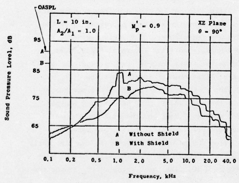
Figure 2.9b. Effect of Shield on Sound Pressure Spectrum at 90° for 10 Inch Augmentor Wing Model.
