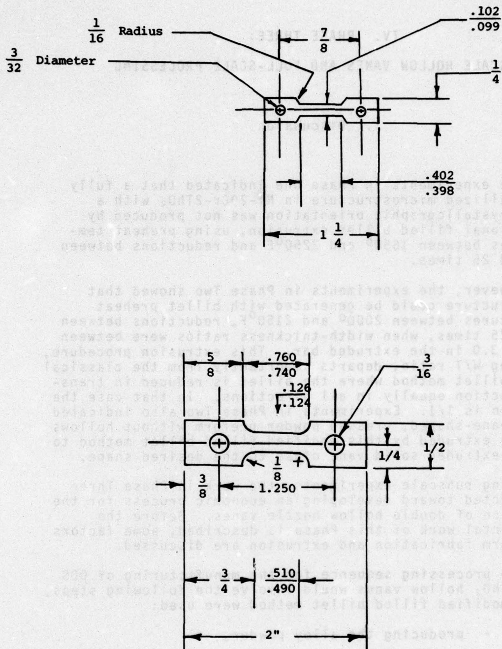
FIGURE 10. SKETCH OF MECHANICAL TEST SPECIMENS IN PHASE TWO
