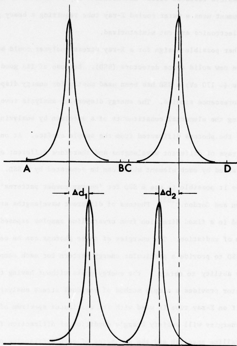
FIGURE 7.2 Illustration of the operation of the single exposure apparatus. a) Stress-free sample b) Sample with compressive stress.
