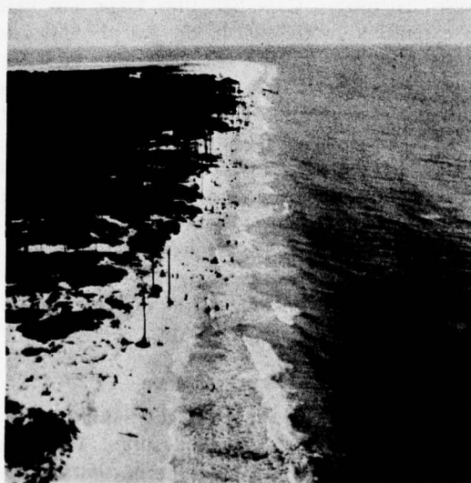
Figure 2.60 Active Beach Erosion Has Moved the Shoreline into Timbered Areas at Cape San Blas, St. Joseph Spit.
