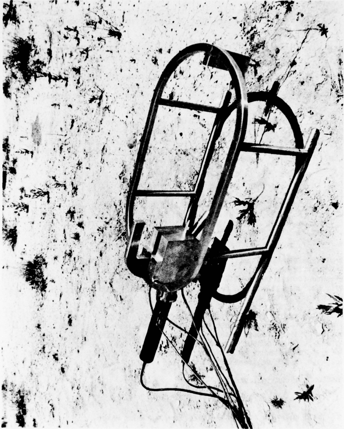
Figure 1. Sensor assembly for soil skin moisture determinator. The moisture at the soil surface affects the quantity of light from the laser source which is received by oblique scattering at the detector.
