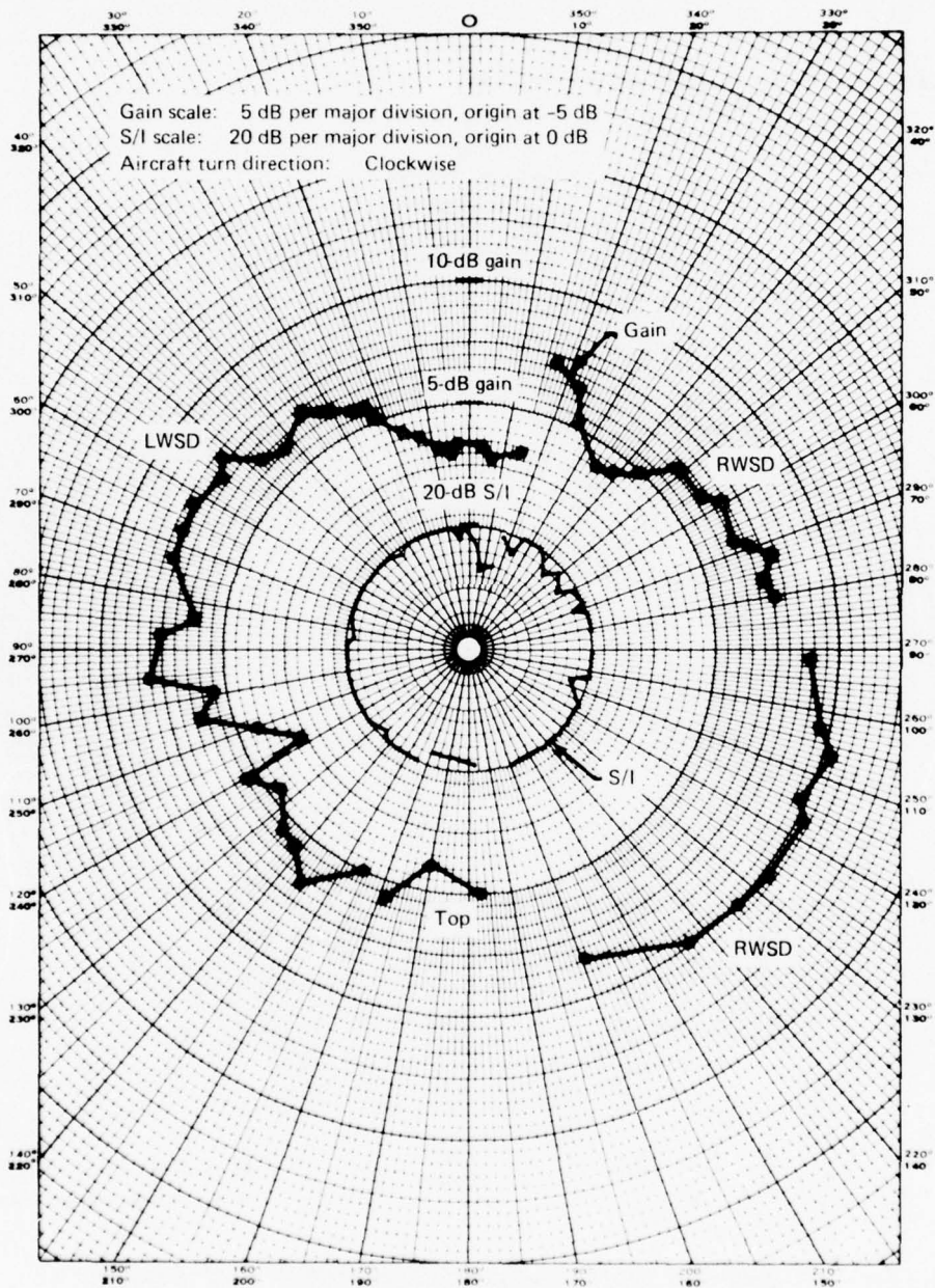
Figure 6-5. Three-Element Slot-Dipole Antenna System Gain and S/I, November 21, 1974, Elevation Angle = 19^\circ
