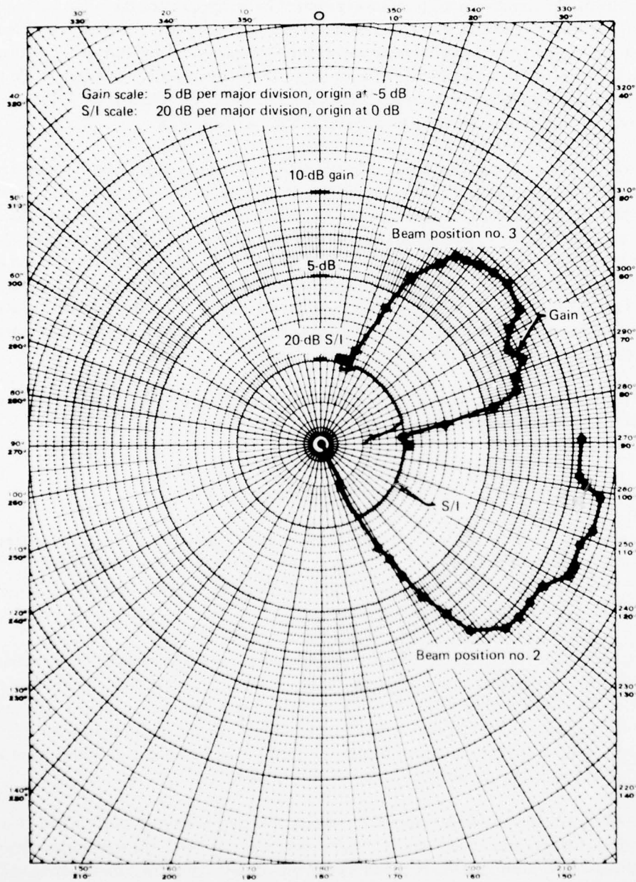
Figure 6-11. Phased-Array Antenna Gain and S/I, October 29, 1974, Elevation Angle = 16^\circ
