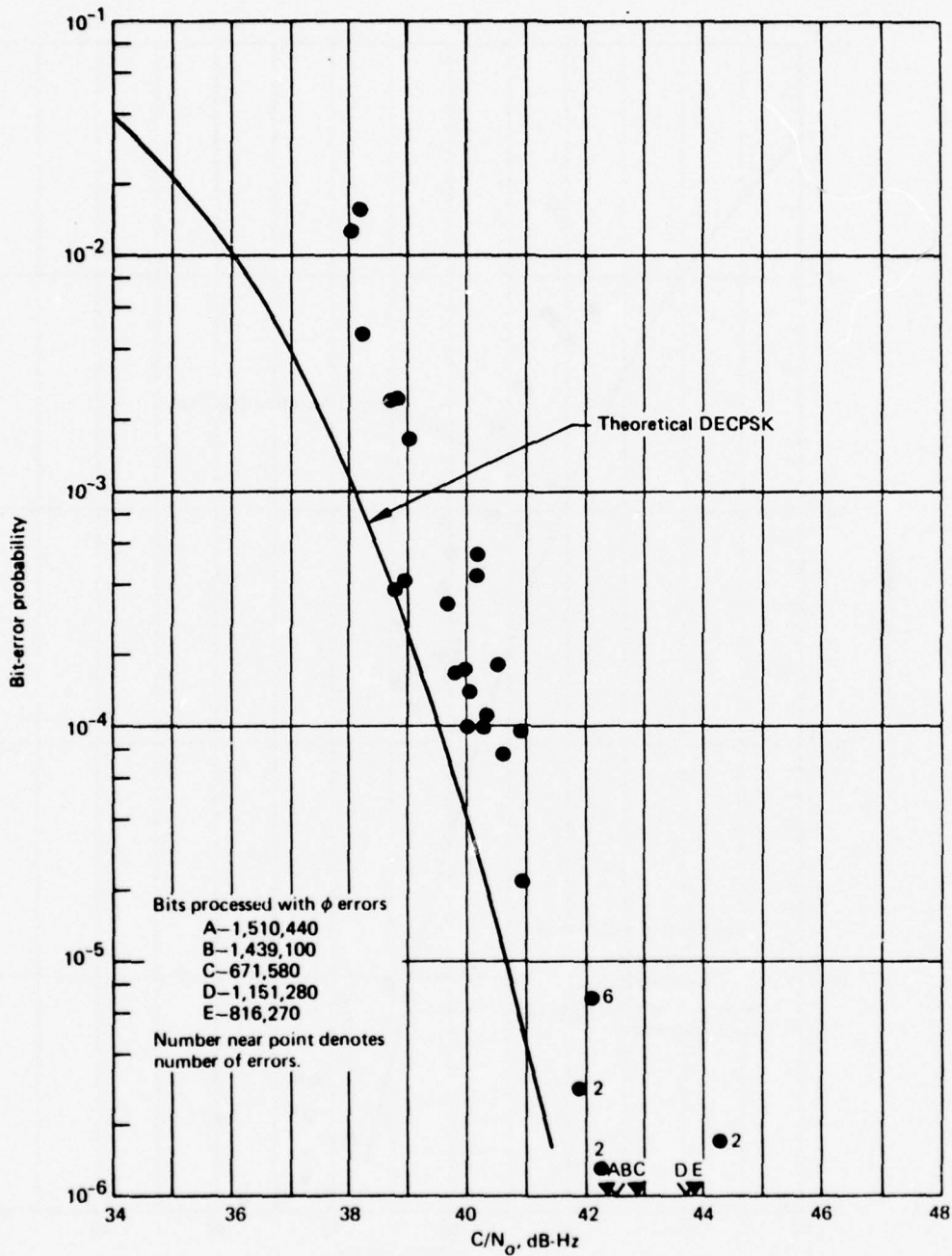
Figure 5-8. Bit Error Rate Performance of Hybrid No. 1 DECPSK Demodulator, 1200 bit/s, Type I Tests
