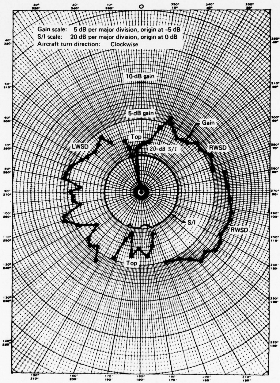
Figure 6-4. Three-Element Slot-Dipole Antenna System Gain and S/I, March 25, 1975, Elevation Angle = 15°
