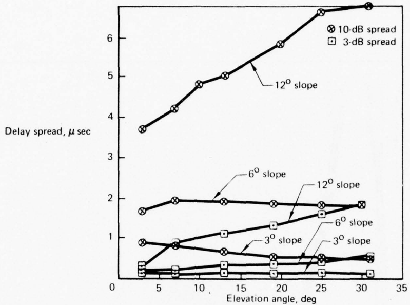
Figure 4-22. Model Predicted Delay Spread – Horizontal Polarization
