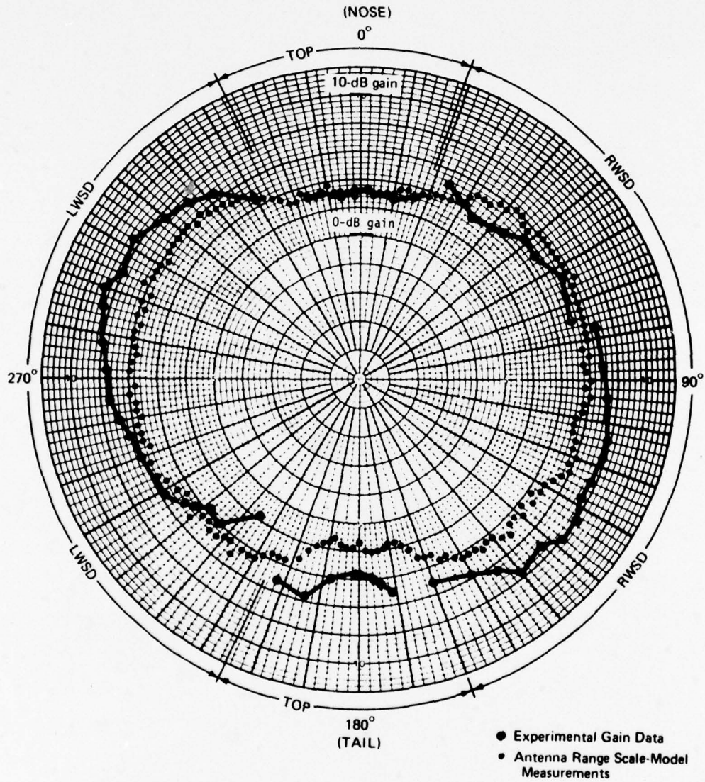
Figure 6-6. Slot-Dipole-System Composite Gain at 20° Elevation
