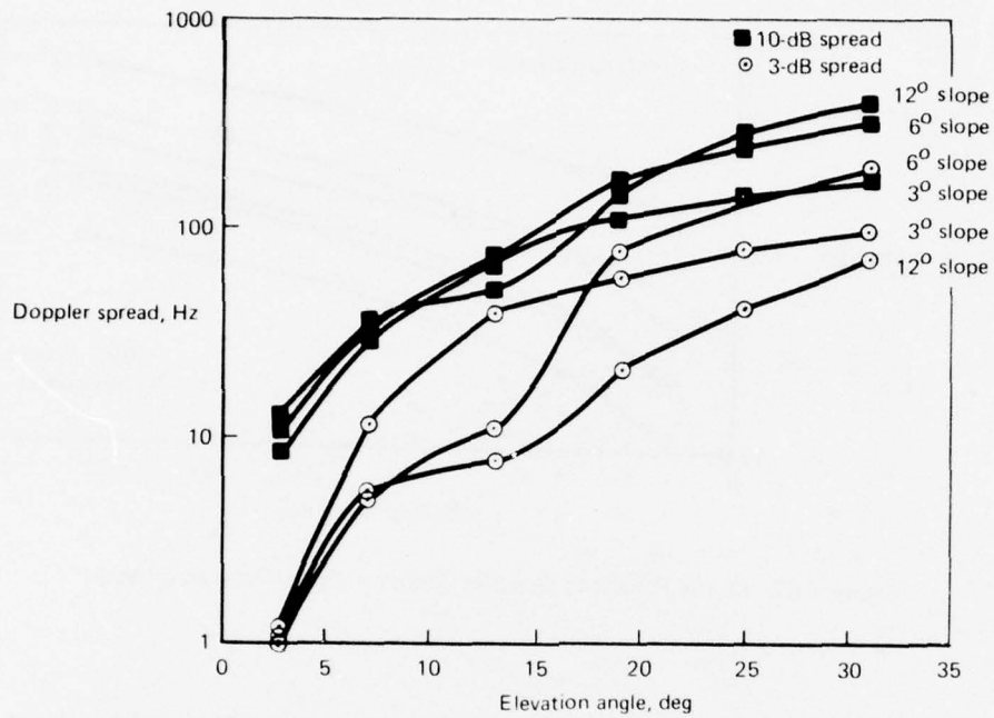
Figure 4-25. Model Predicted Doppler Spread – Horizontal Polarization, In-Plane Geometry
