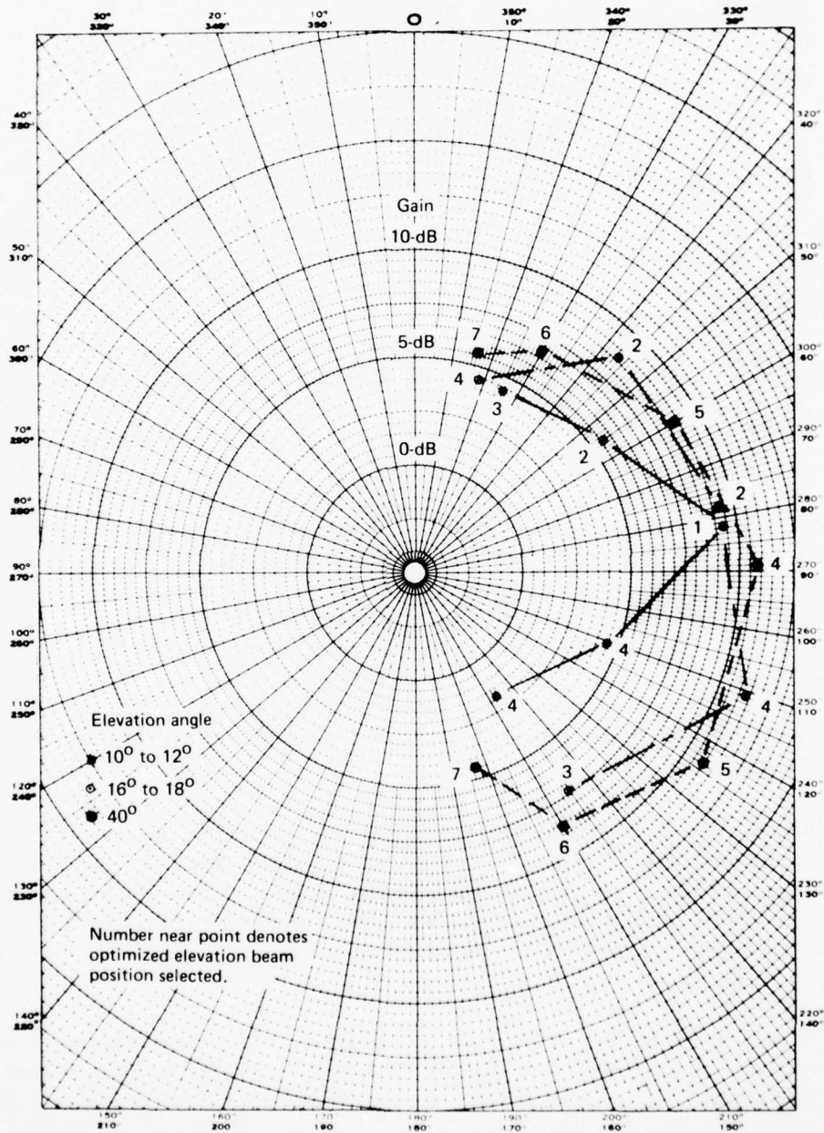
Figure 6-9. Phased-Array Gain Data for "Straight-Line" Tests
