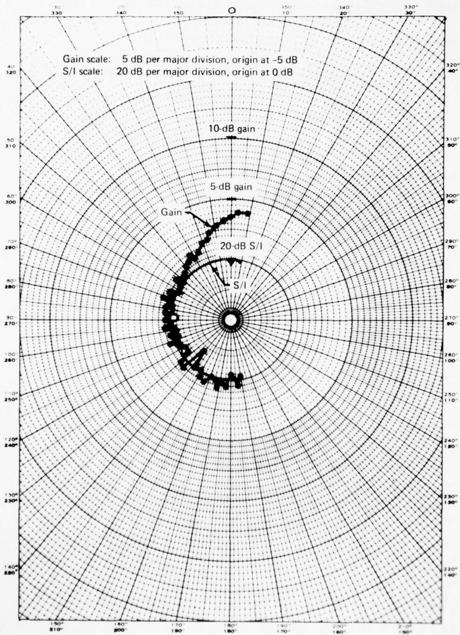
Figure 6-15. Patch Antenna Gain and S/I, October 29, 1974, Elevation Angle = 16°
