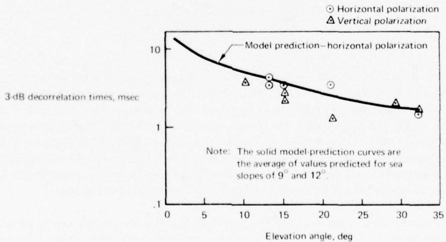
Figure 4-16. Oceanic Decorrelation Time Results – Cross-Plane Geometry
