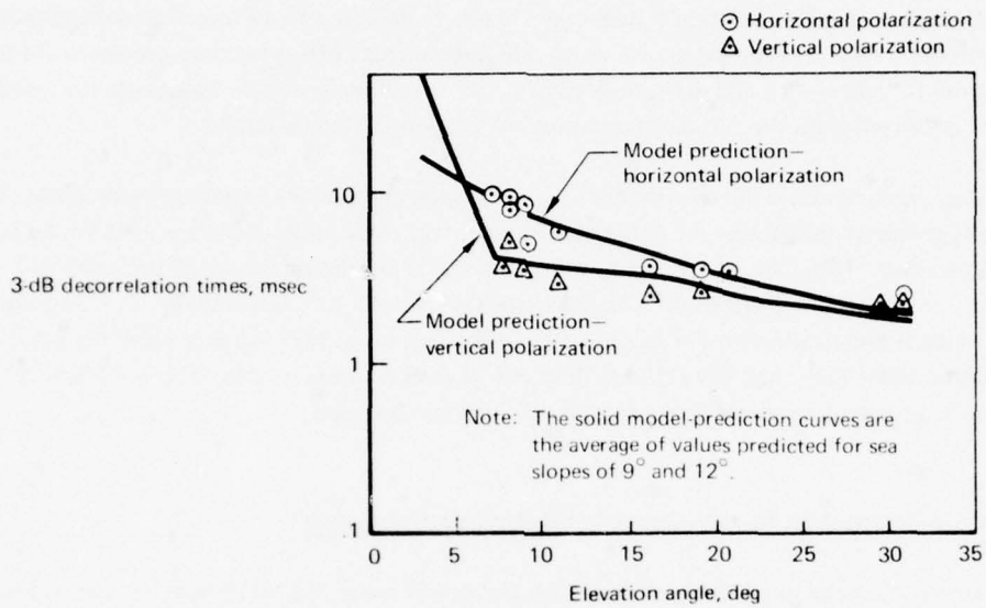
Figure 4-15. Oceanic Decorrelation Time Results – In-Plane Geometry
