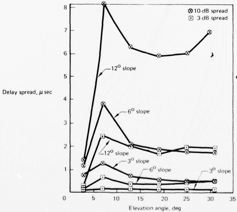
Figure 4-23. Model Predicted Delay Spread – Vertical Polarization
