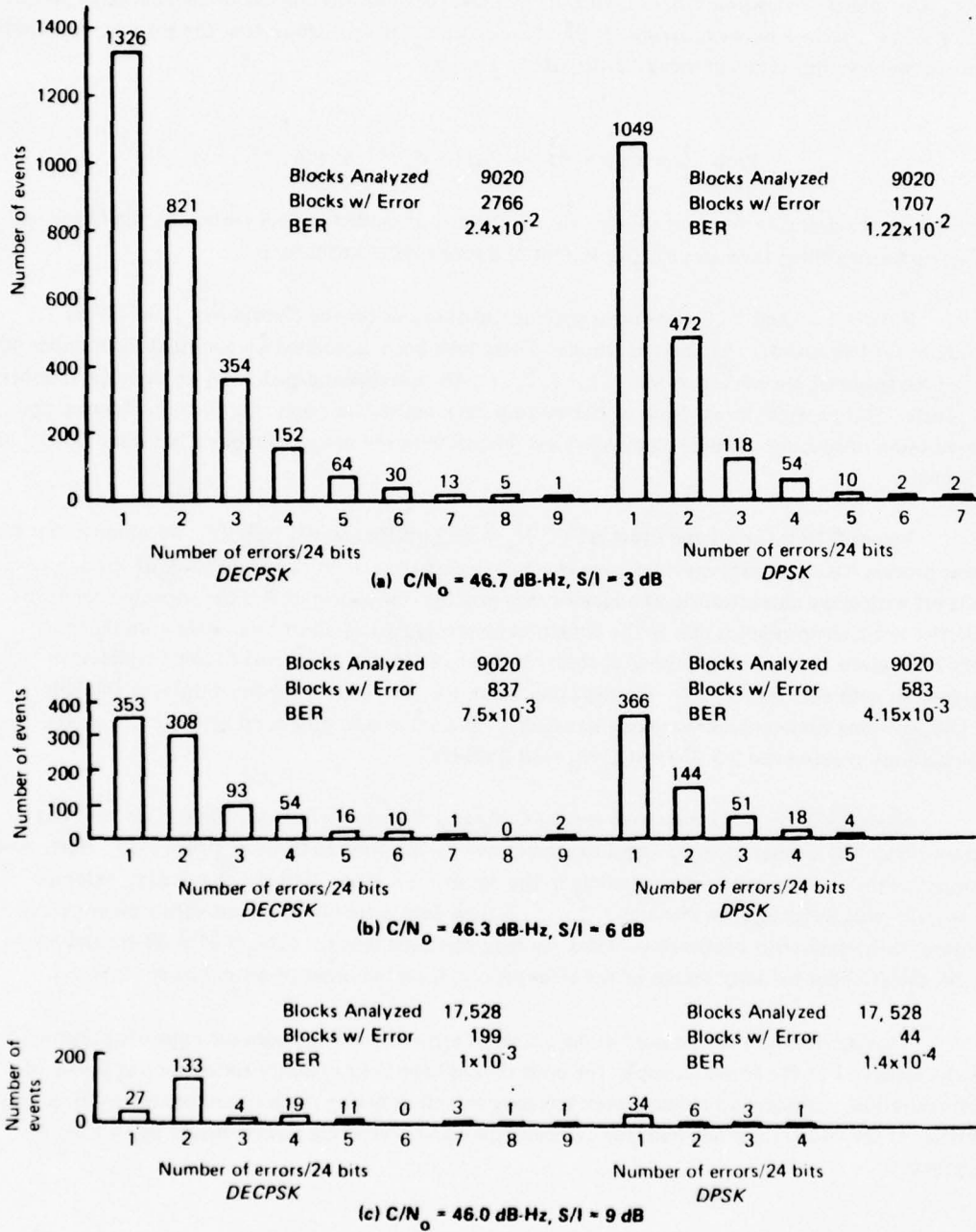
Figure 5-18. Type II Block Error Histograms
