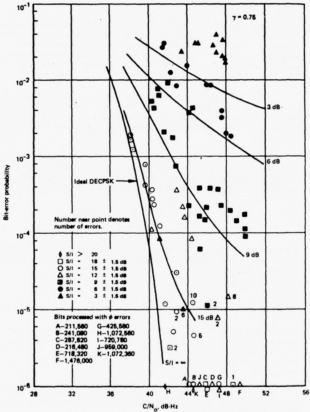
Figure 5-13. Bit Error Rate Performance of Hybrid No. 1 DECPSK Demodulator, 1200 bit/s, Type II Tests
