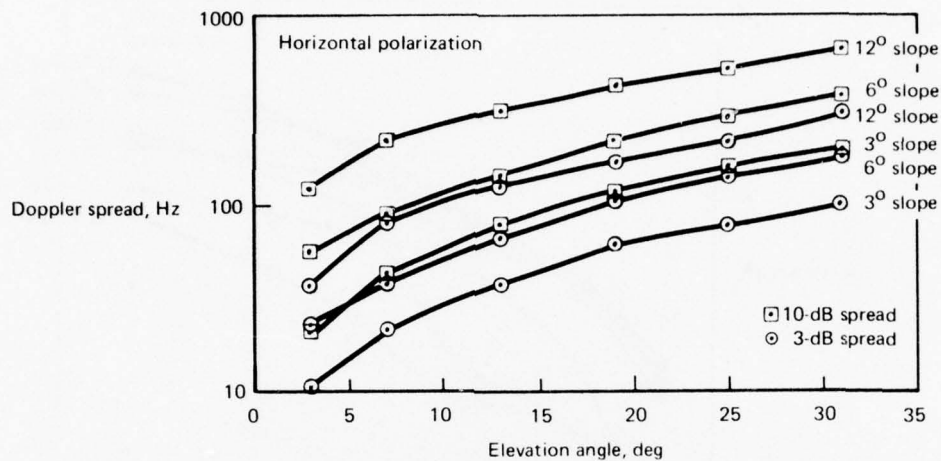
Figure 4-27. Model Predicted Doppler Spread – Cross-Plane Geometry
