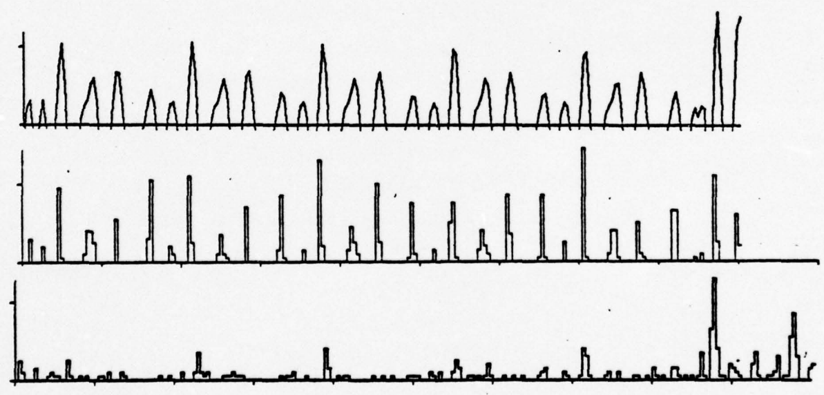
Figure 31. /o/-POHs from neuron 710827/11 (lower curve in (a) and (b) ) and Model 08/13/76 (middle curve in (a) and (b) ) and corresponding segment from the ROC COC2 response, positive values only (upper curve in (a) and (b) ). In (a) the neuron run is 16, the model run is 08/13/76.2/3, and the stimulus is 8A, presented at an intensity of 20 dB attenuation. In (b) the neuron run is 8, the model run is 08/13/76.1/3, and the stimulus is 4A, presented at an intensity of 40 dB attenuation.
