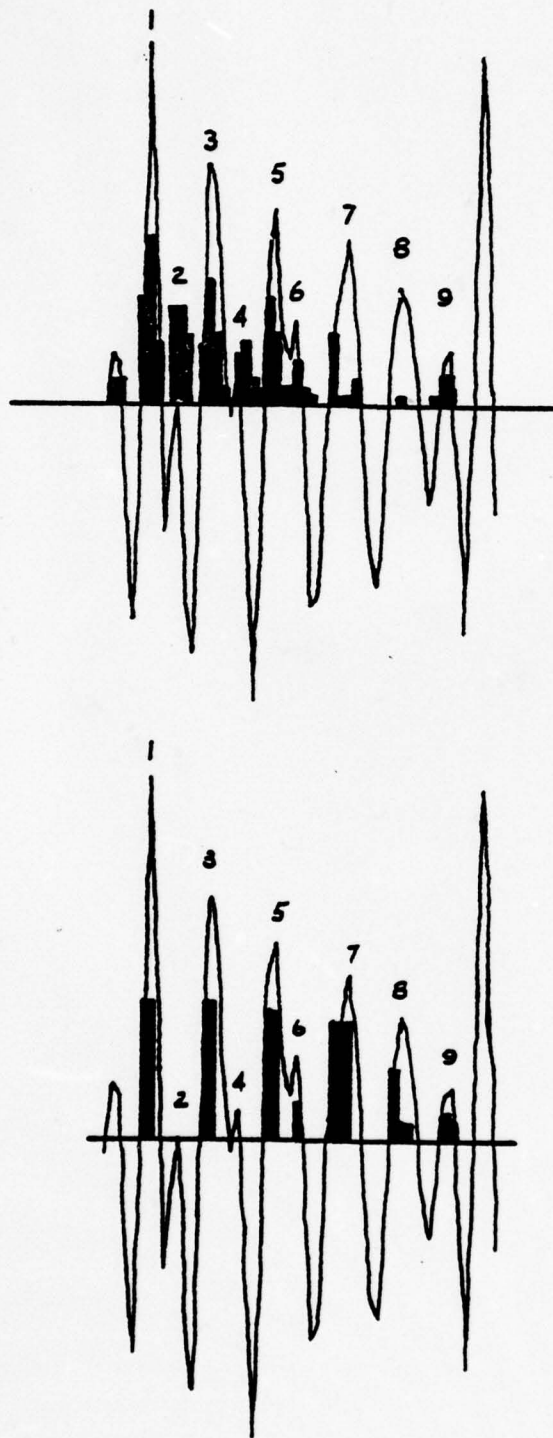
Figure 7. A pitch period of the vowel /ɪ/ superimposed on a typical corresponding segment of a 40 dB attenuation /ɪ/-POH. (a) is neuron 710827, run 9. (b) is model run 08/13/76.1/4.
