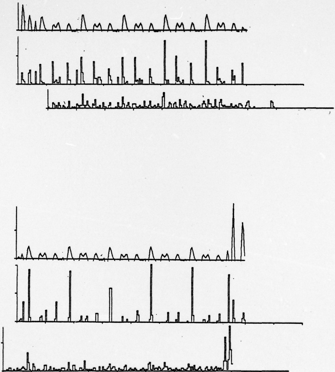
Figure 46. /u/-POHs from neuron 710827/11 (lower curve in (a) and (b) ) and Model 08/13/76 (middle curve in (a) and (b) ) and corresponding segment from the ROC COC2 response, positive values only (upper curve in (a) and (b) ). In (a) the neuron run is 17, the model run is 08/13/76.2/4, and the stimulus is 8B, presented at an intensity of 20 dB attenuation. In (b) the neuron run is 9, the model run is 08/13/76.1/4, and the stimulus is 4B, presented at an intensity of 40 dB attenuation.
