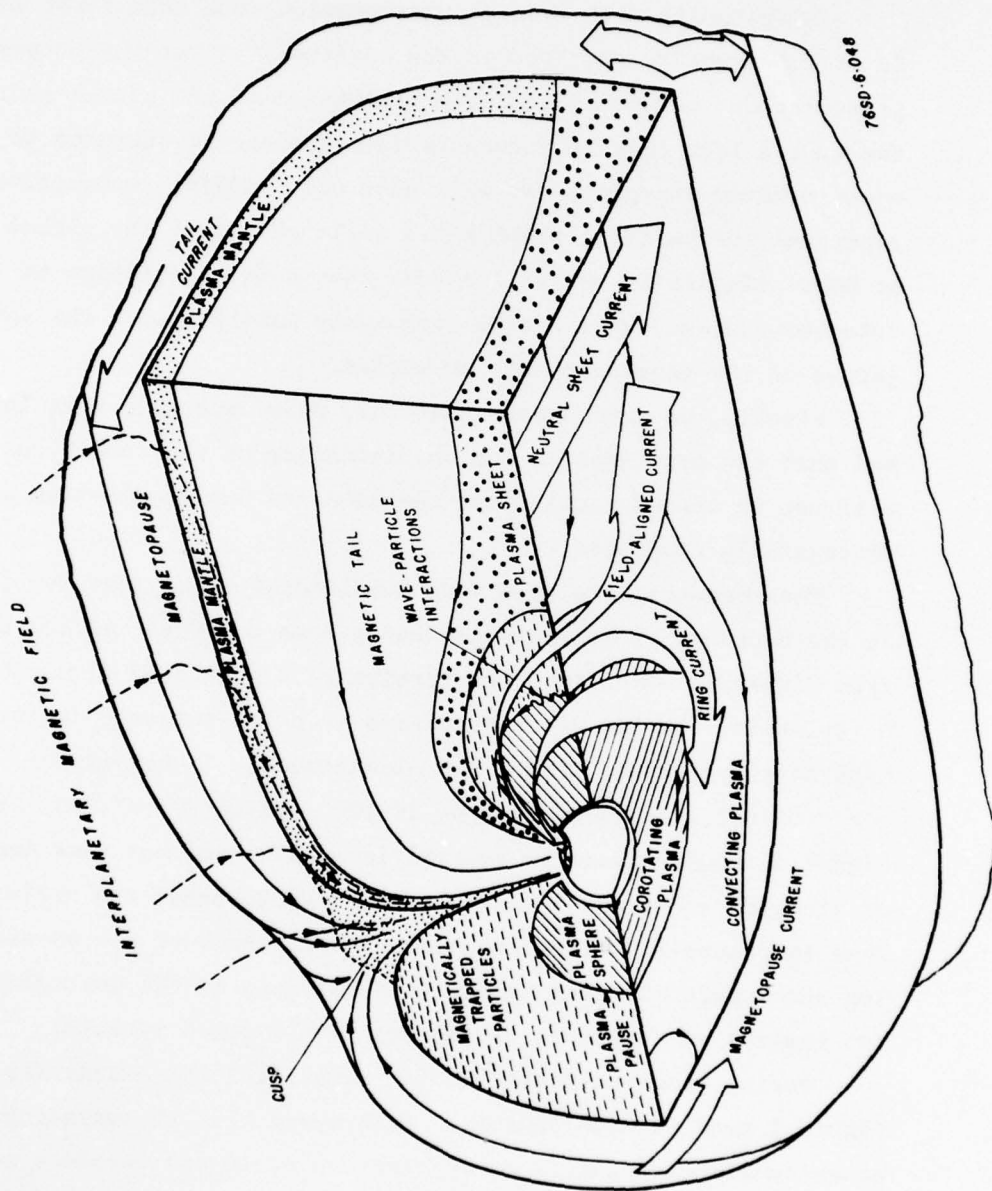
Figure 1. Magnetosphere (Heikkila)
