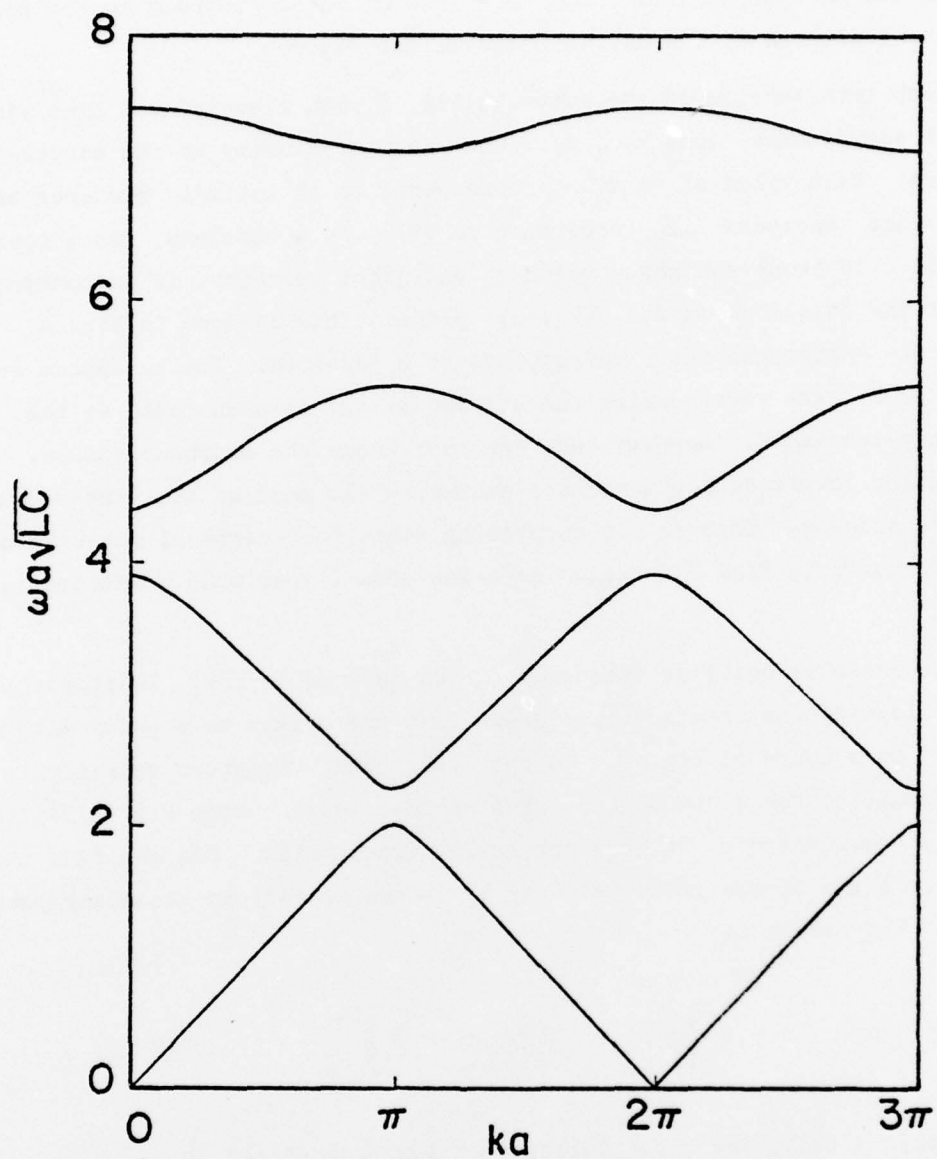
Figure 4. Plot of frequency \omega as a function of propagation constant k , showing the passband-stopband structures. The curves for negative k and \omega can be obtained by reflections with respect to the horizontal and vertical coordinate axes.
