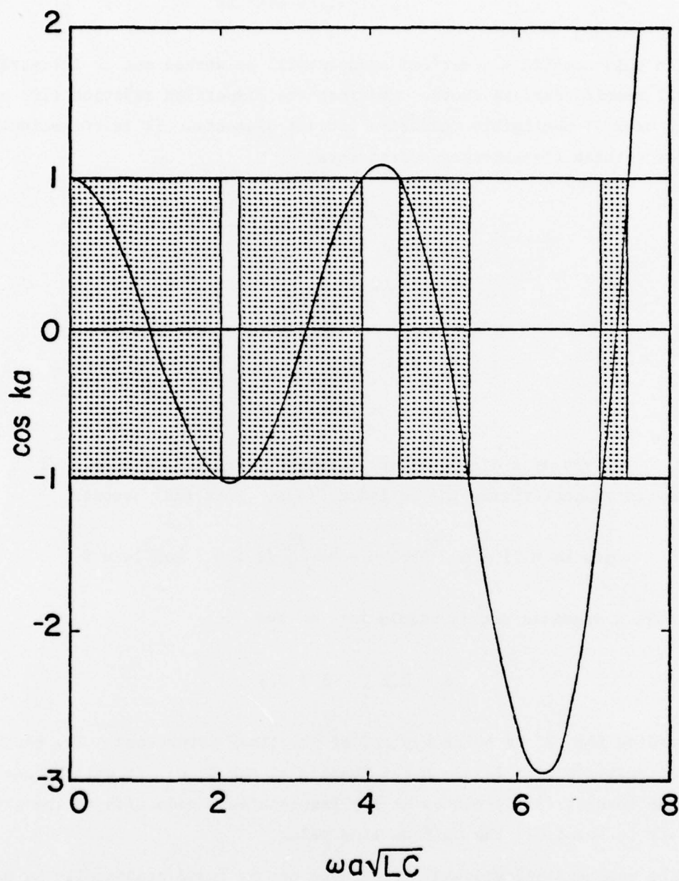
Figure 3. Graphical solution of the dispersion relation (42) of a periodically loaded transmission line in the (\cos ka, \omega) plane. The frequency ranges for which -1 \leq \cos ka \leq 1 correspond to the passbands (dotted areas).
