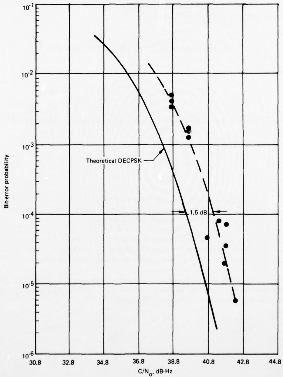
Figure 5-4. Laboratory Baseline Bit-Error-Rate Performance of FAA CPSK Demodulator, (DECPSK Mode), 1200 bps, August 1974
