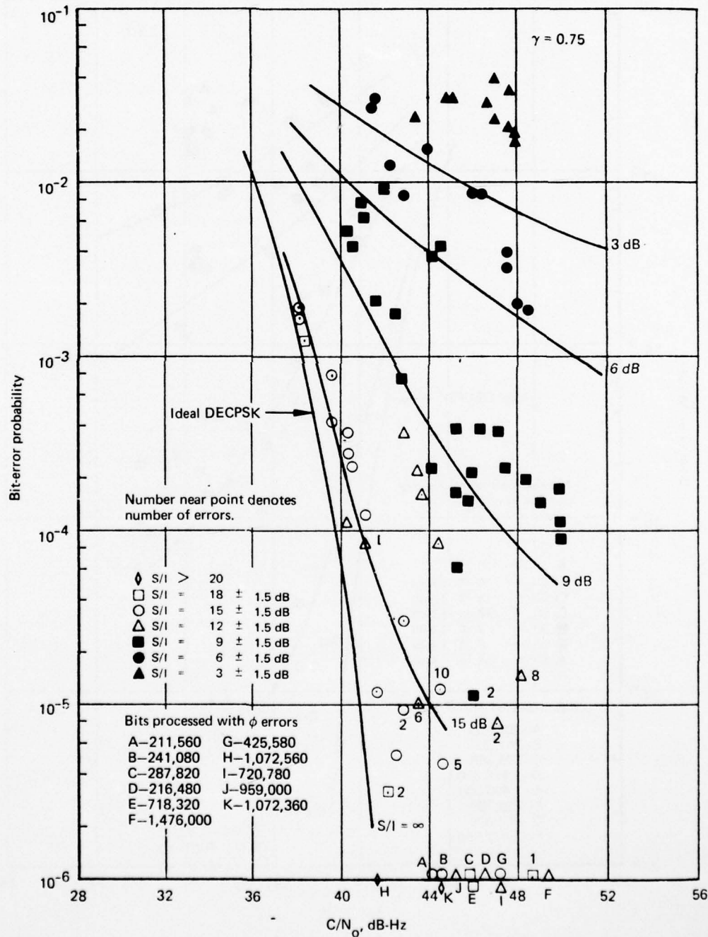
Figure 5-11. Bit-Error-Rate Performance of Hybrid No. 1 DECPSK Demodulator, 1200 bps, Type II Tests
