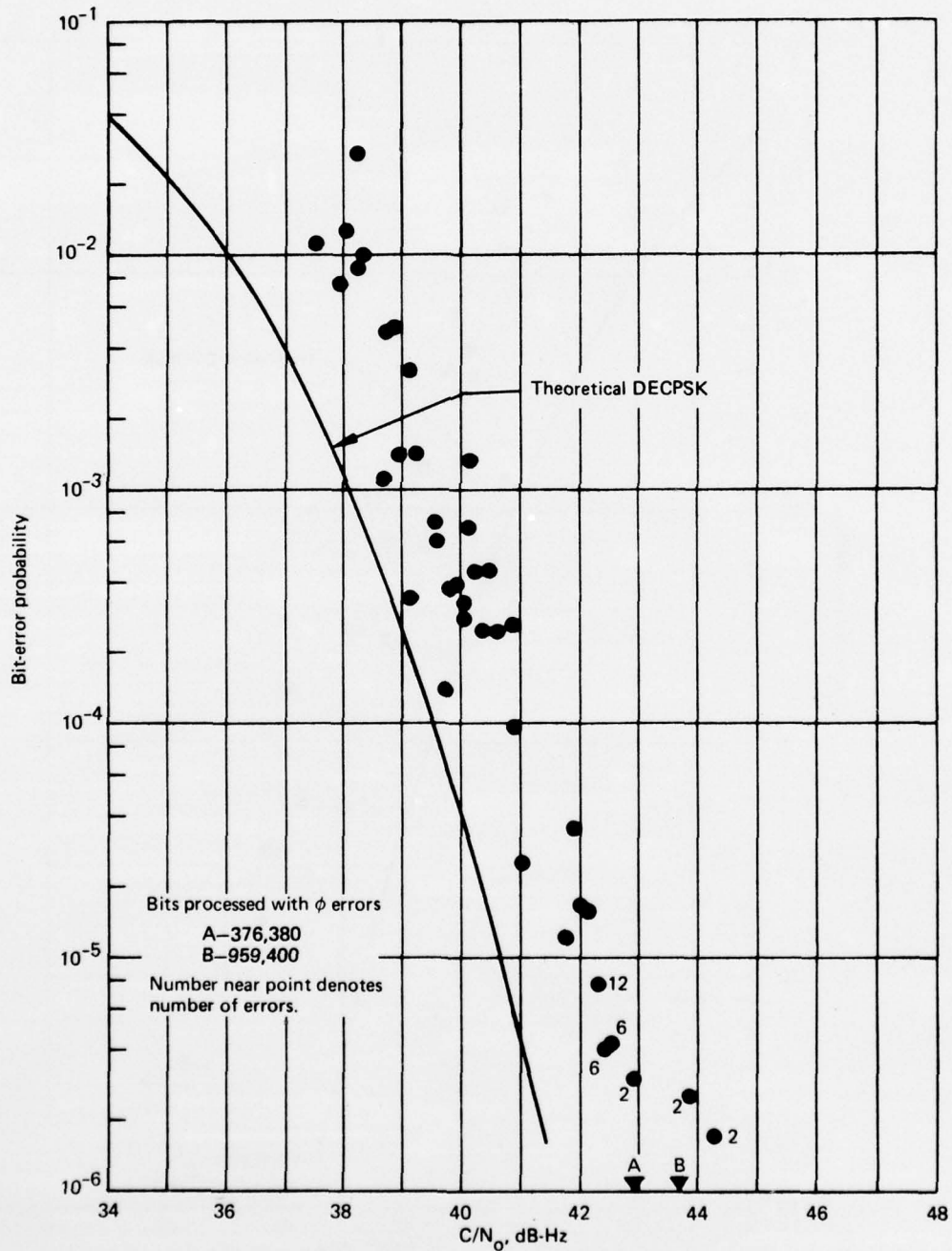
Figure 5-8. Bit-Error-Rate Performance of FAA CPSK Demodulator (DECPSK Mode), 1200 bps, Type I Tests
