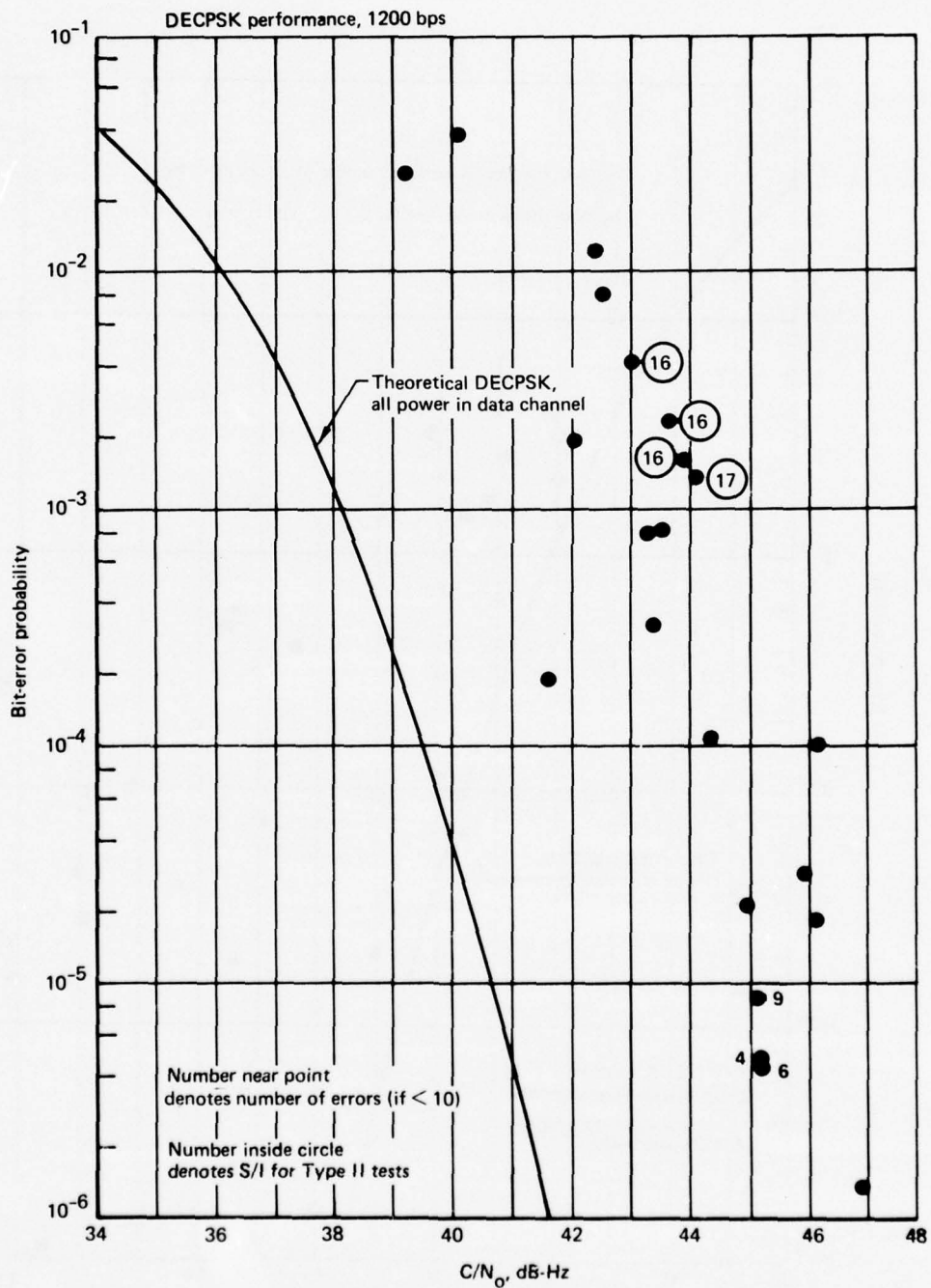
Figure 5-24. Bit-Error-Rate Performance, Hybrid No. 2 Modem, Hybrid Voice and Data Mode, 1200 bps
