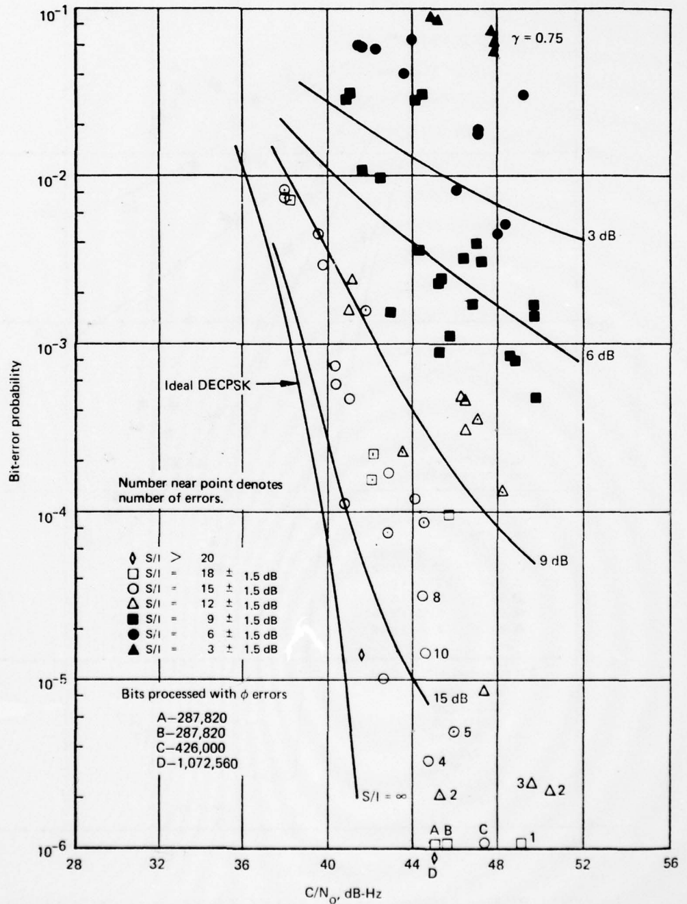
Figure 5-13. Bit-Error-Rate Performance of NASA DECPSK Demodulator, 1200 bps, Type II Tests
