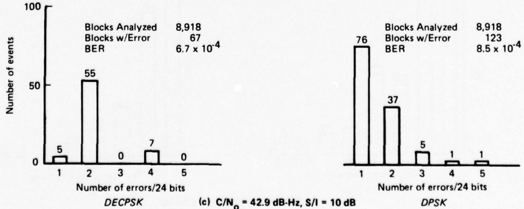
Figure 5-19. Type II Block-Error Histograms, C/N_0 = 43 dB-Hz
