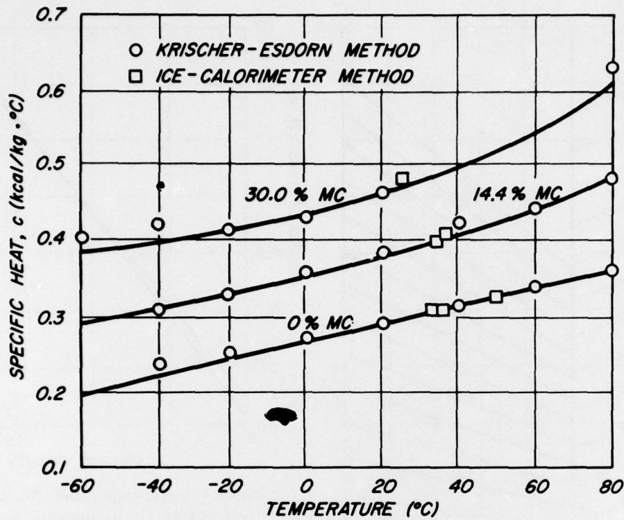
Figure 2.--Specific heat, c , versus temperature, with moisture content as the parameter.
