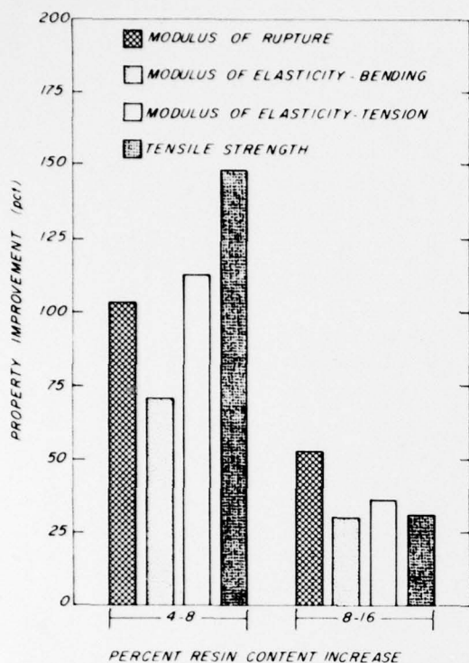
Figure 5. -- Relationship of wet property improvements of medium-density boards to doubled amounts of phenolic resin. (M 144 687)
