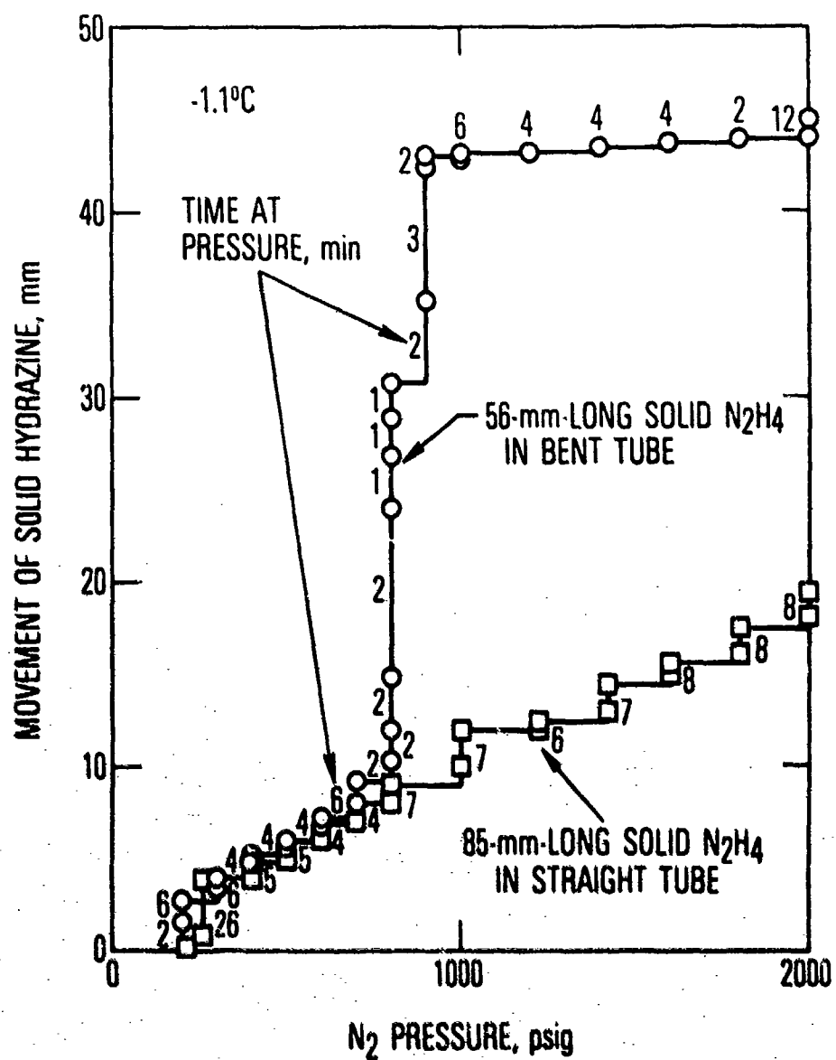
Fig. 7. Movement of pure solid hydrazine in 0.25-in. straight and 120^\circ -bent stainless-steel tubes at -1.1^\circ C ( +30^\circ F )
