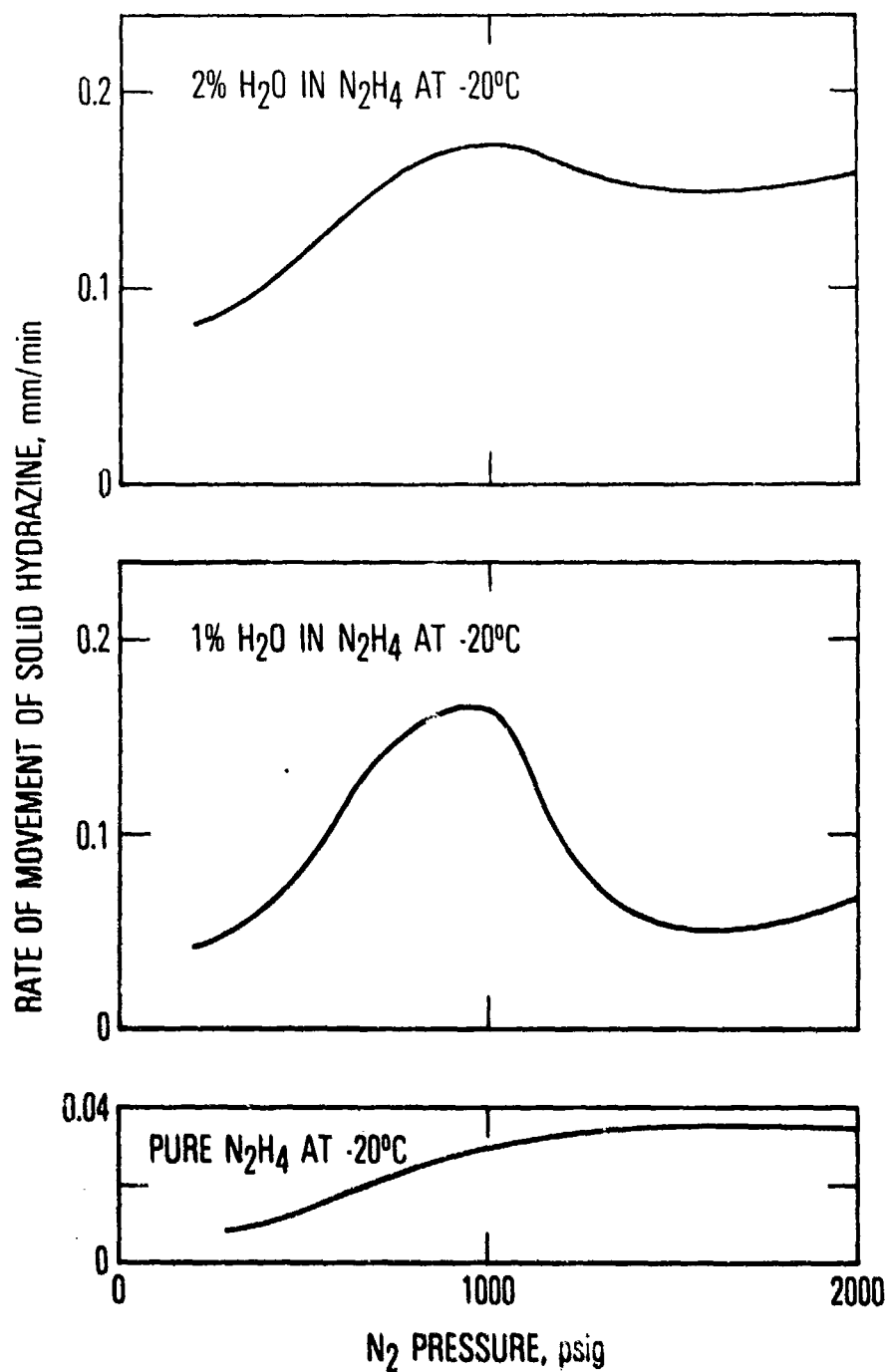
Fig. 11. Rate of movement of solid hydrazine containing various amounts of water in 0.25-in. 120°-bent stainless-steel tubes at -20°C (-4°F)
