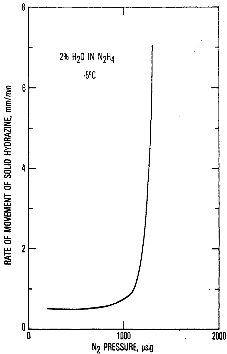
Fig. 15. Rate of movement of solid hydrazine containing 2% water in 0.25-in. 120°-bent stainless-steel tube at -5°C (+23°F)
