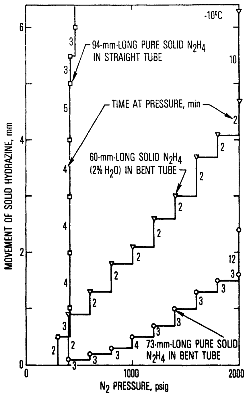
Fig. 12. Movement of solid hydrazine containing various amounts of water in 0.25-in. straight and 120°-bent stainless-steel tubes at -10^\circ C ( +14^\circ F )
