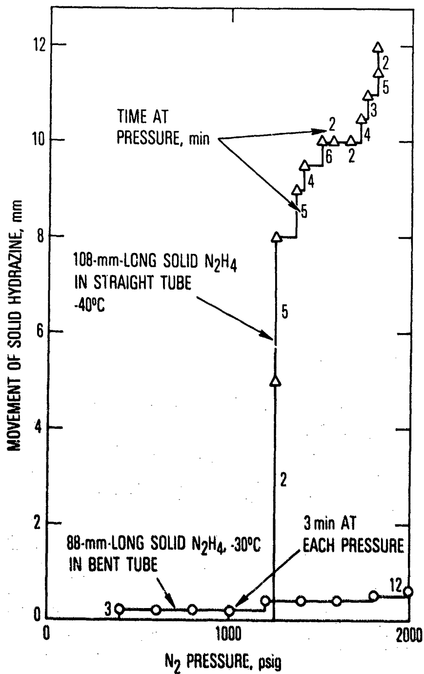
Fig. 4. Movement of pure solid hydrazine in 0.25-in. straight and 120^\circ -bent stainless-steel tubes at -40^\circ C ( -40^\circ F ) and -30^\circ C ( -22^\circ F )
