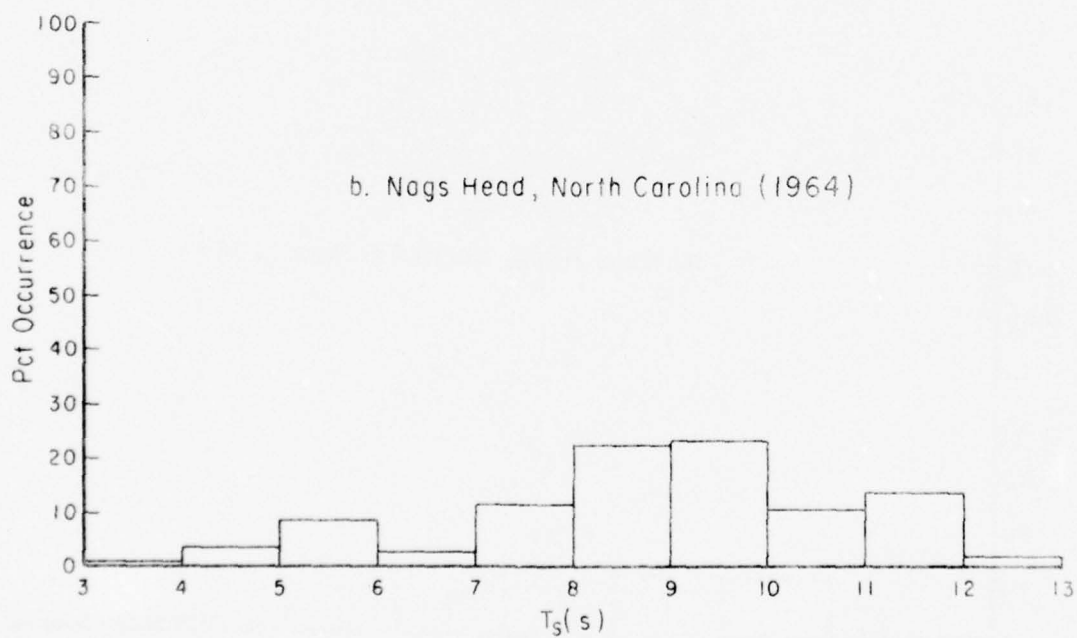
Figure 22. Distribution of wave periods during tests at Ventnor and Nags Head.
