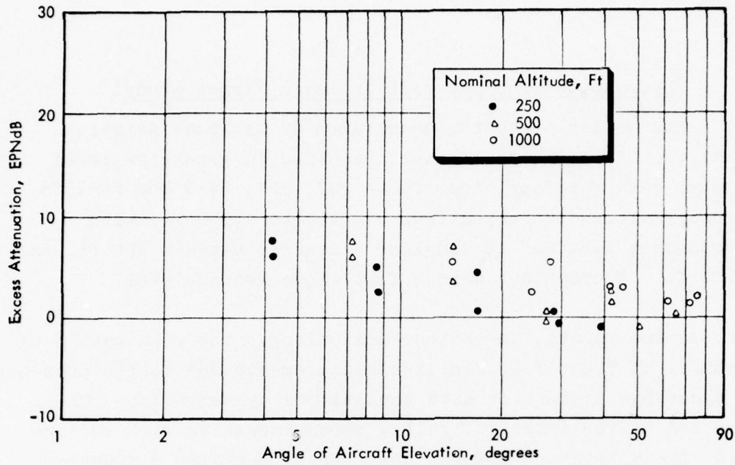
FIGURE 3(a). EXCESS ATTENUATION-707-320B AIRCRAFT (HYDROSPACE REFERENCE 10)
