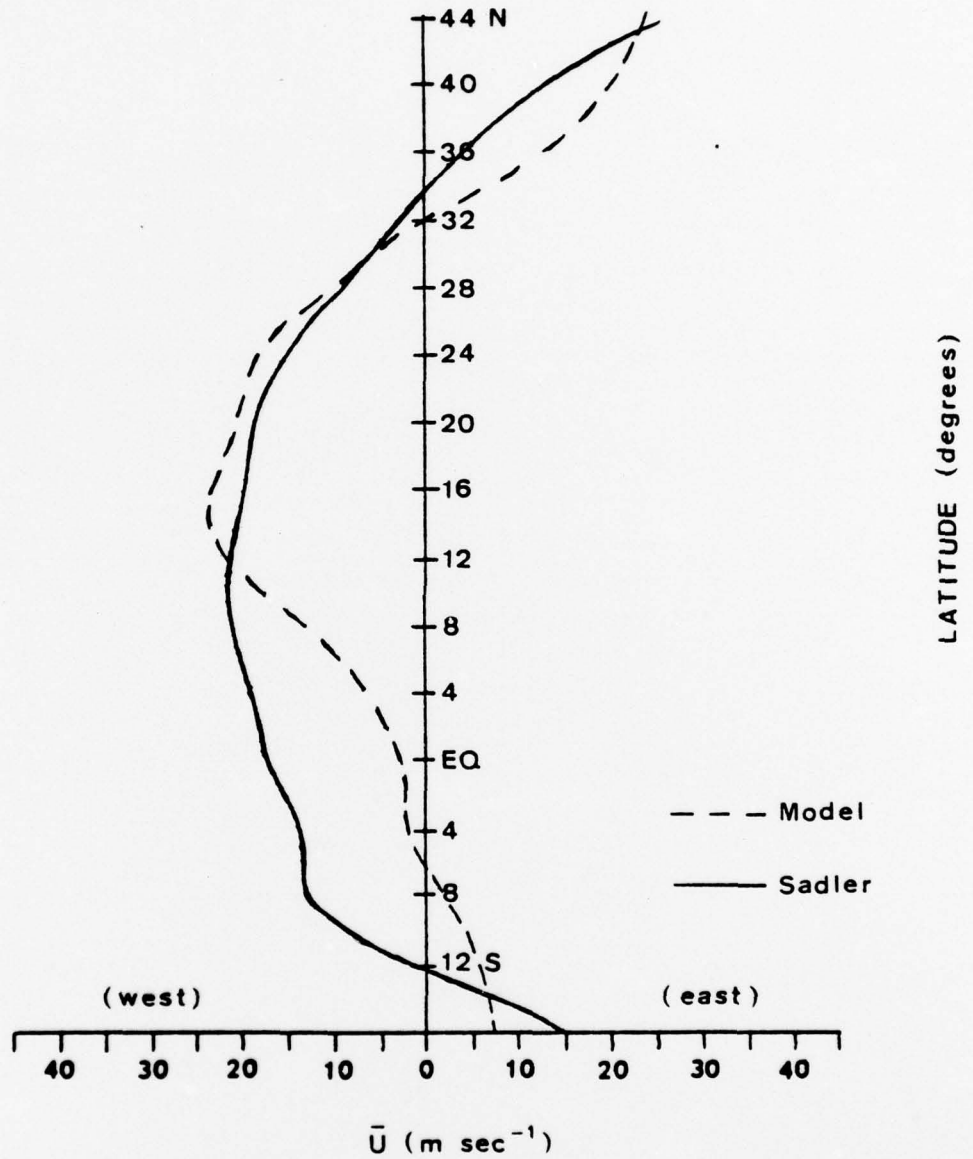
Figure 8: Simulated zonal wind at 250 mb vs. observed zonal wind at 200 mb for July, no topography. Units are \text{m sec}^{-1} .
