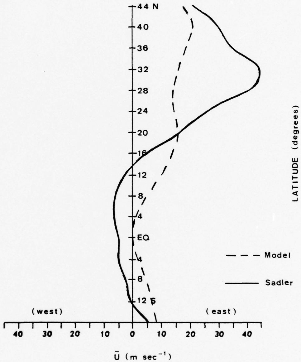
Figure 6: Simulated zonal wind at 250 mb vs. observed zonal wind at 200 mb for January, no topography. Units are m sec -1 .
