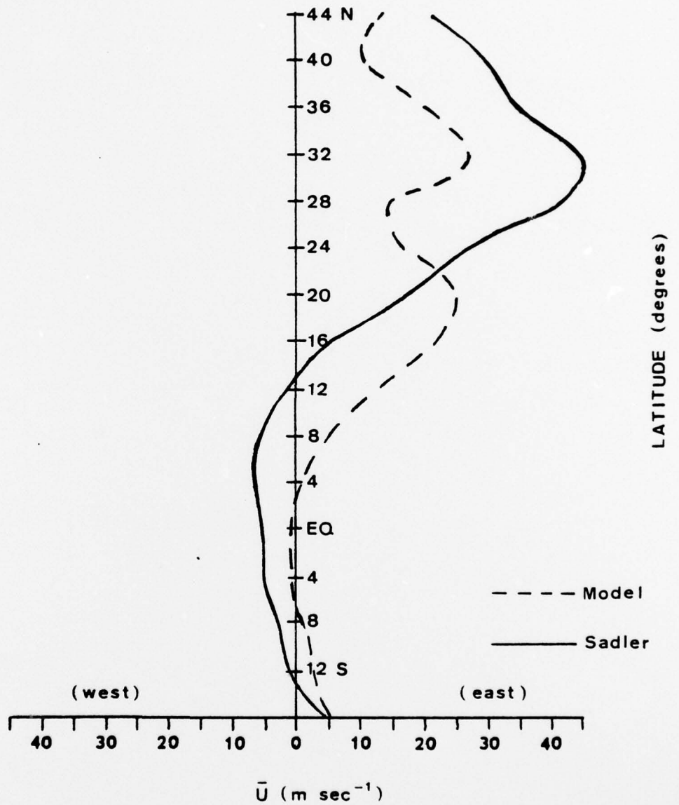
Figure 10: Simulated zonal wind at 250 mb vs. observed zonal wind at 200 mb for January with topography. Units are \text{m sec}^{-1} .
