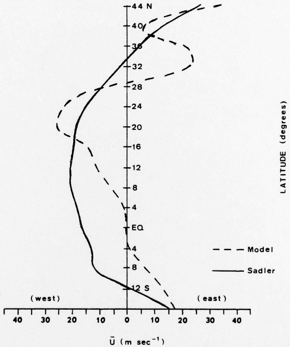
Figure 12: Simulated zonal wind at 250 mb vs. observed zonal wind at 200 mb for July, with topography. Units are m sec -1 .
