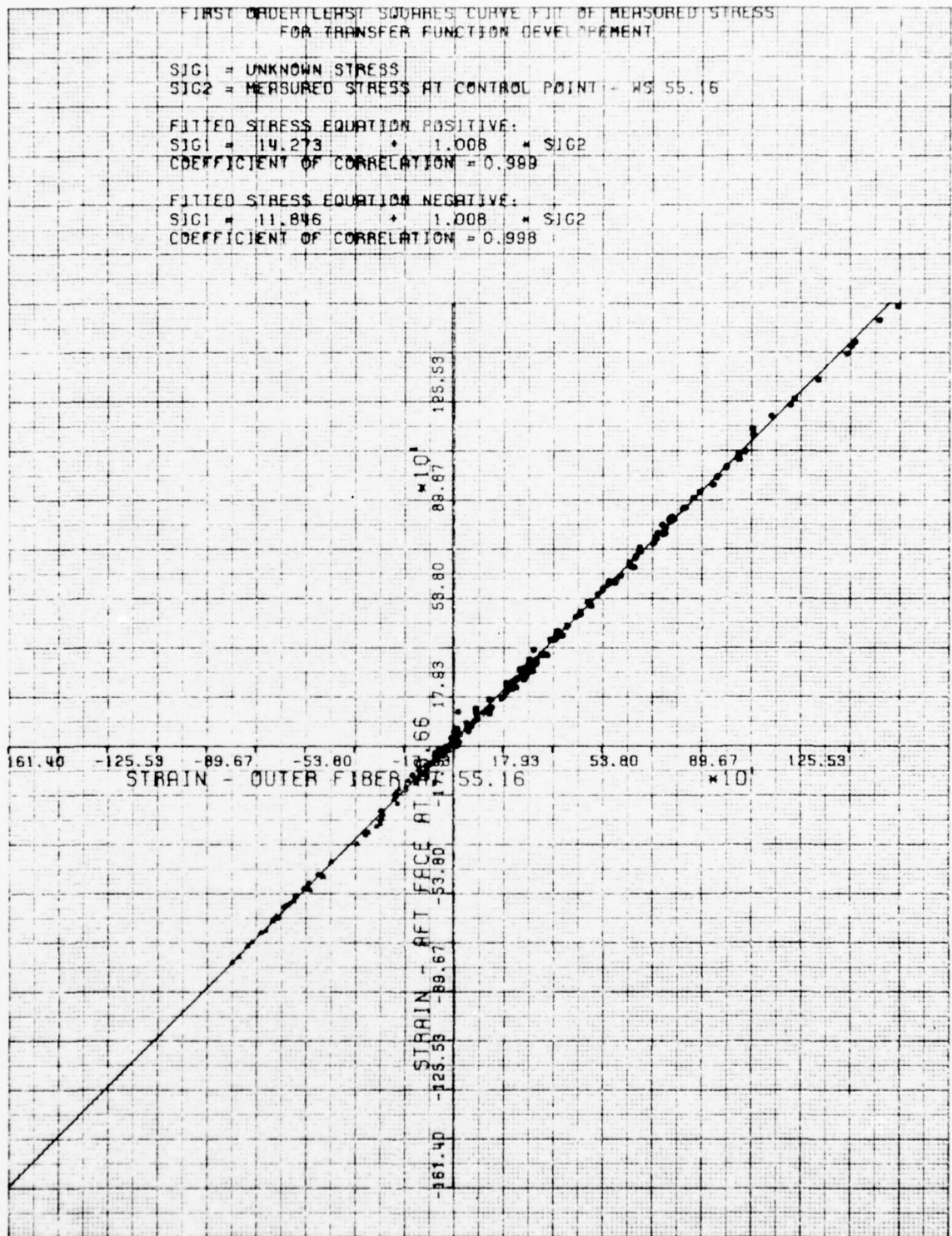
Figure 5 Transfer Function Development 11
