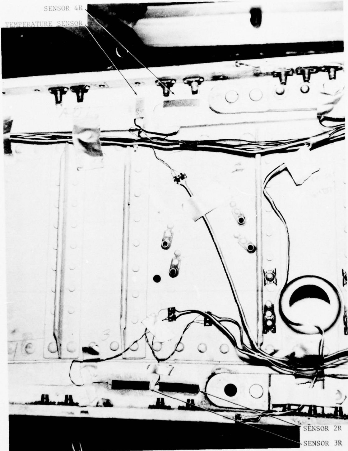
Figure 2 Inboard Front Spar Installation 6
