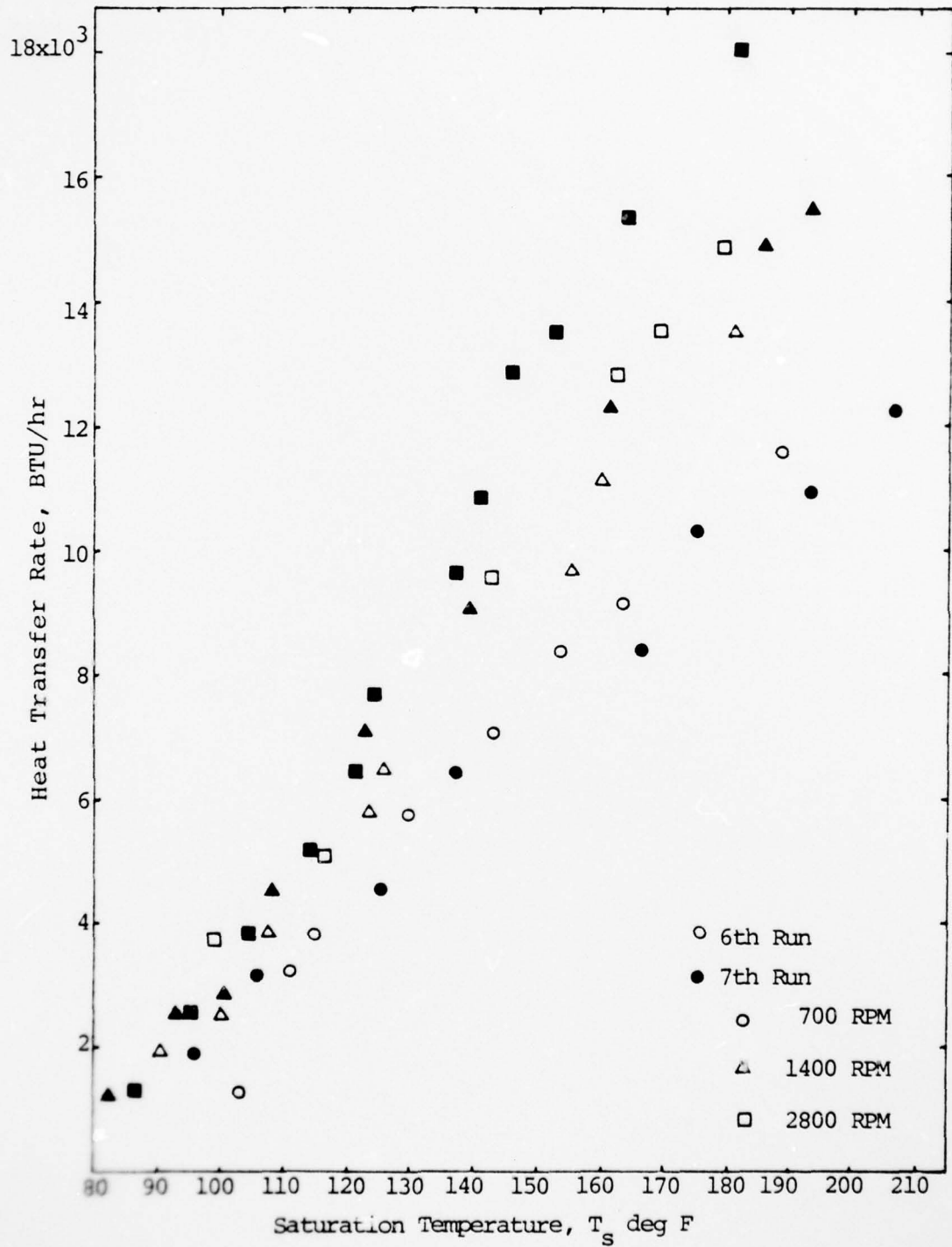
Figure 19. Heat Transfer Rate Versus Saturation Temperature for Truncated Cone Condenser with 0.5 Degree Half Angle
