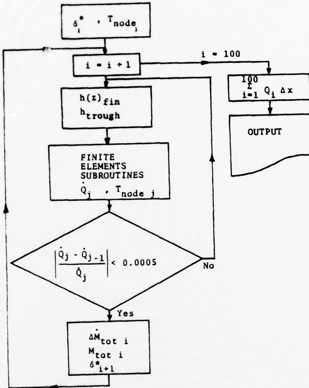
Figure 9. Computer Program Flowchart of Two-Dimensional Conduction Analysis of Corley [16]
