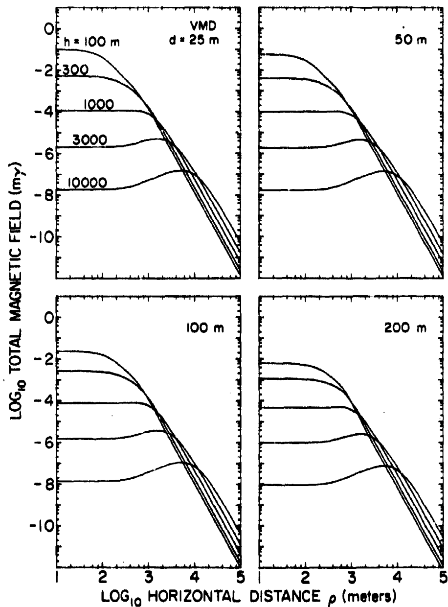
Figure III-3. Variation of the amplitude of the 1 Hz total magnetic field produced at depth d in an infinitely deep sea ( \sigma = 4 mho/m) by a vertical magnetic dipole of unit moment at height h above the sea surface.
