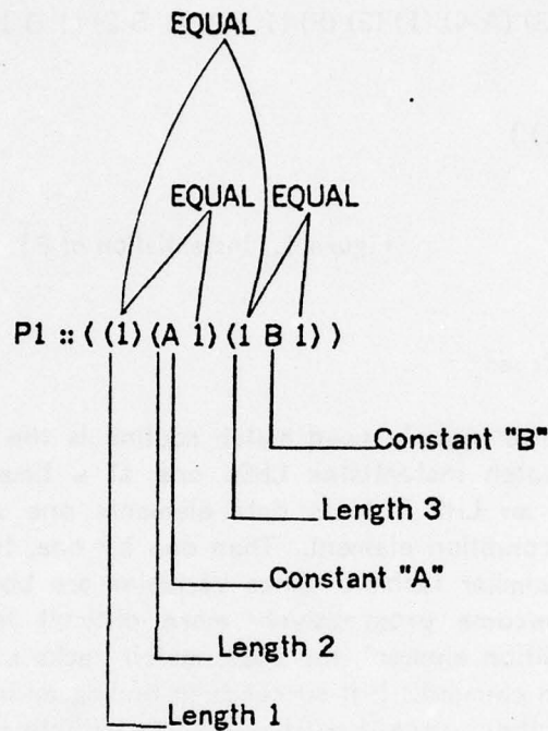
Figure 2. Characteristics of instantiations of P1.
