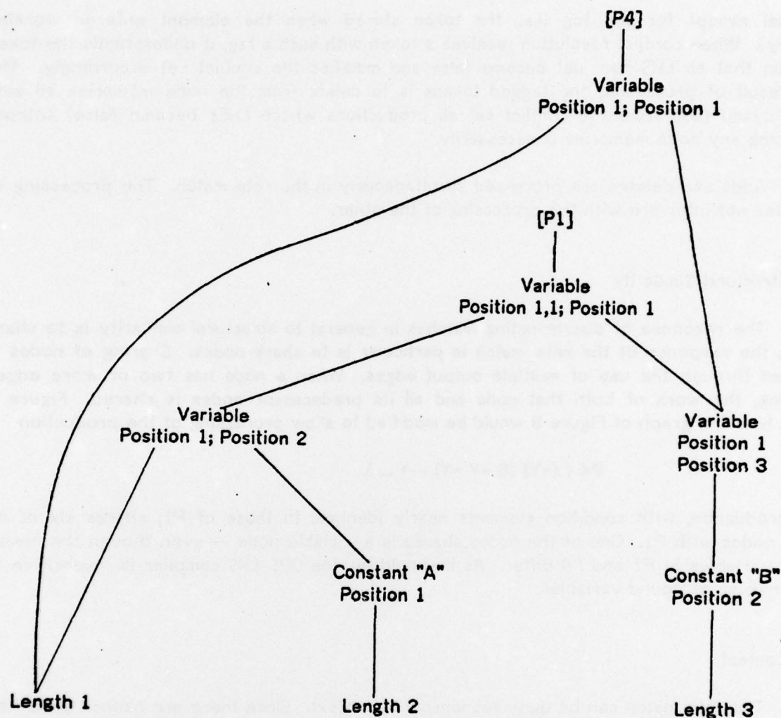
Figure 4. Match routine for P1 and P4.
