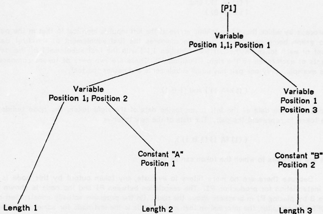
Figure 3. Match routine for P1.
