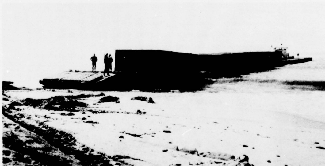
Figure 37. Top-lift loader with container negotiating causeway beach ramp during Lo/Ro operation.
