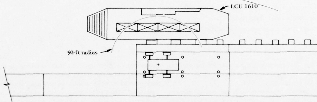
Figure 44. LCU operation at pierhead. Note crane operating radius of 50 feet (15 m) reaching four containers.
