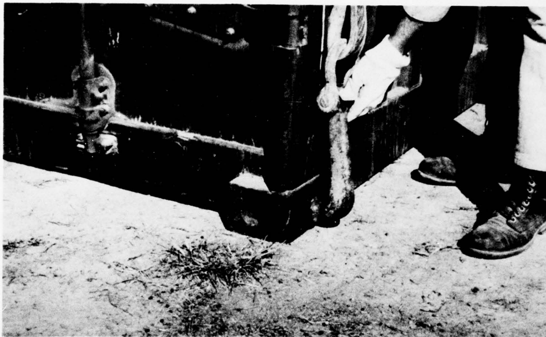
Figure 20. Modified bulb hook on sling spreader being inserted into corner fitting of container.
