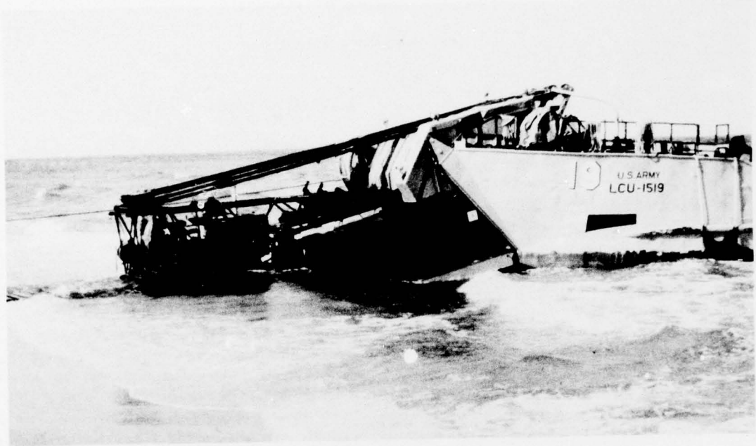
Figure D-1. P&H 9125-TC crane (tactically disassembled ) being delivered to beach in LCU.
