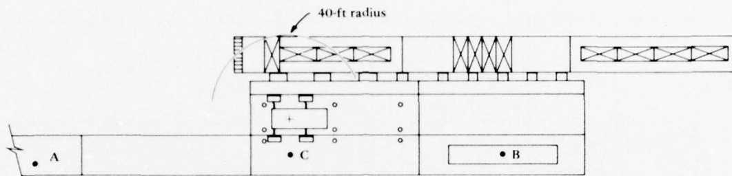
Figure 33. Schematic of causeway ferry operations at pierhead. Note container loading configuration.
