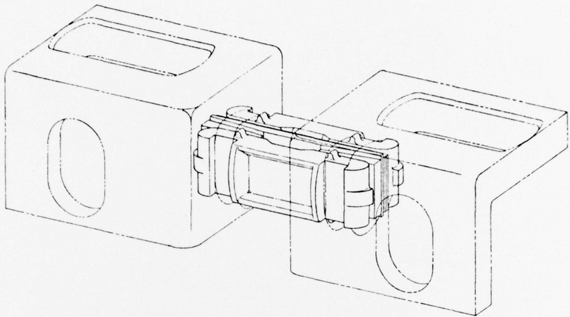
Figure B9. In-place view of assembled coupler.
