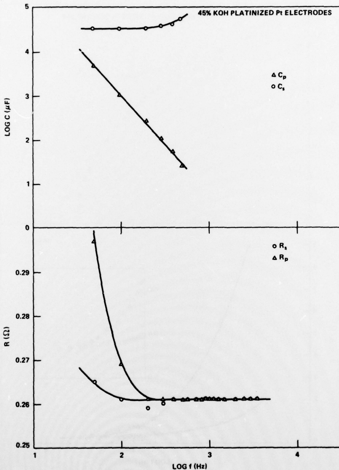
FIG. 5 EQUIVALENT PARALLEL AND SERIES RESISTANCES AND CAPACITANCES VERSUS FREQUENCY OF CONDUCTIVITY CELL FILLED WITH 45% KOH SOLUTION AT 25.0° C USING PLATINIZED Pt ELECTRODES.
