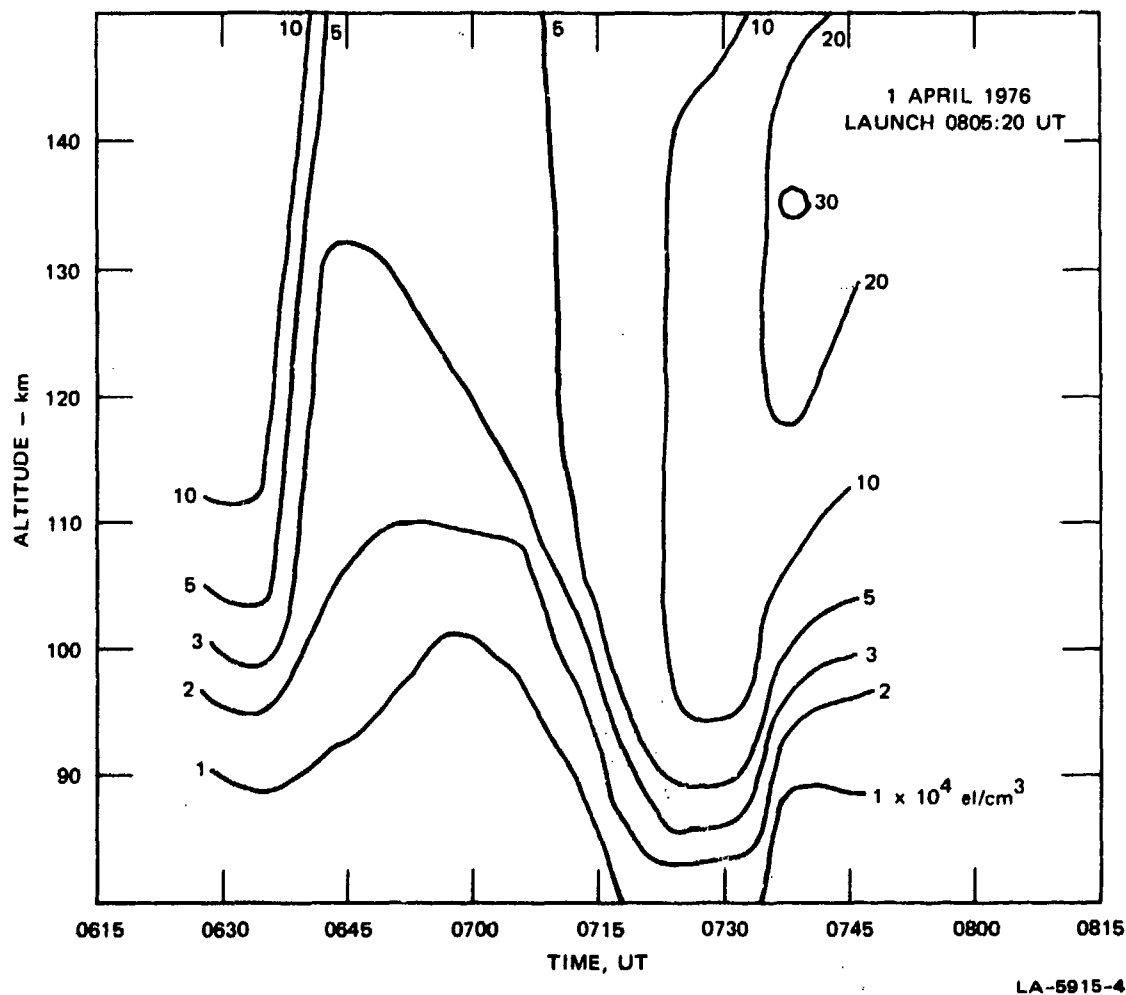
FIGURE 4 BACKGROUND CONTOURS OF ELECTRON DENSITY FOR THE HIRIS EXPERIMENT ON 1 APRIL 1976
