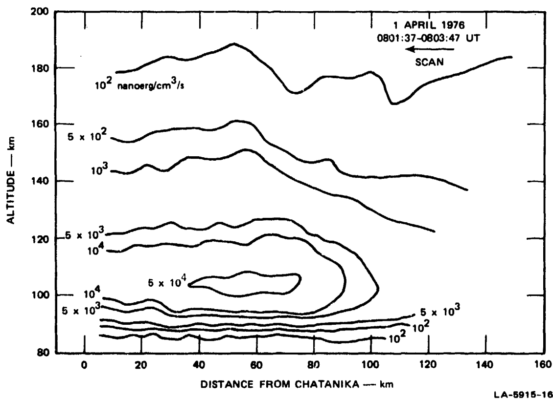
FIGURE 16 VOLUME ENERGY DEPOSITION RATE IN THE VICINITY OF THE HIRIS TRAJECTORY FOR THE PERIOD 0801:37 TO 0803:47 UT, 1 APRIL 1976
