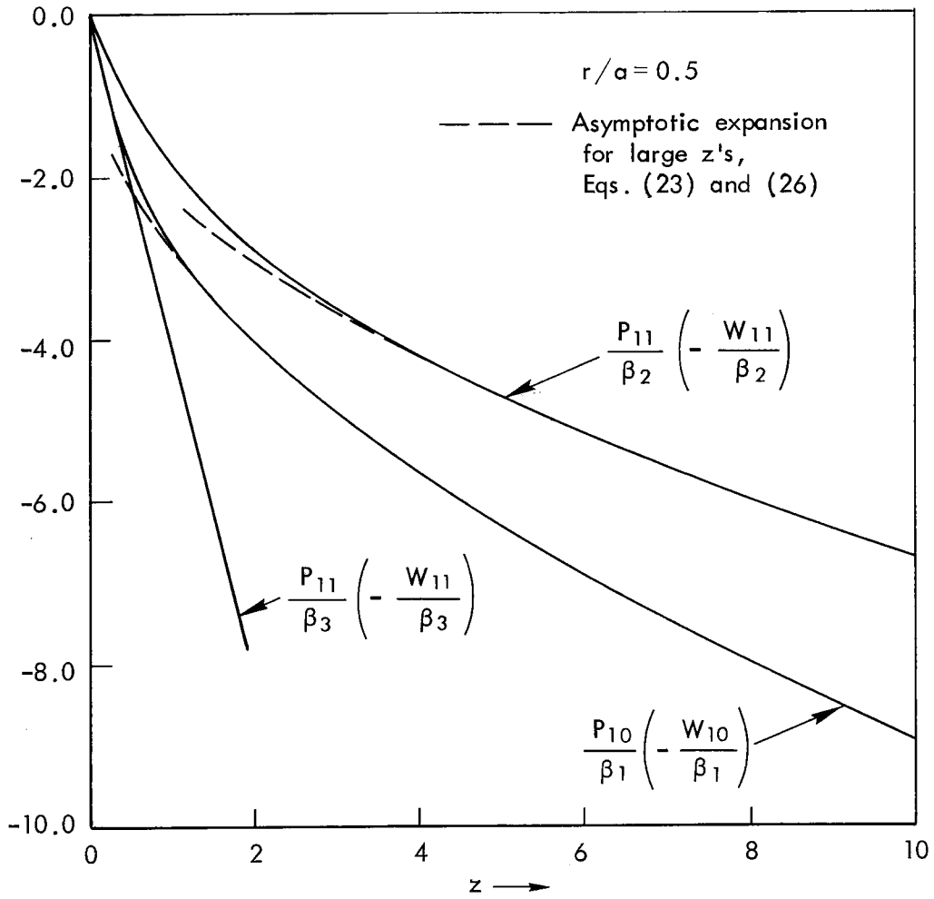
Fig. 8— Displacement effect \frac{W_{10}}{\beta_1} (or -\frac{P_{10}}{\beta_1} ), and secondary flow effect \frac{W_{11}}{\beta_2} (or \frac{P_{11}}{\beta_2} )
