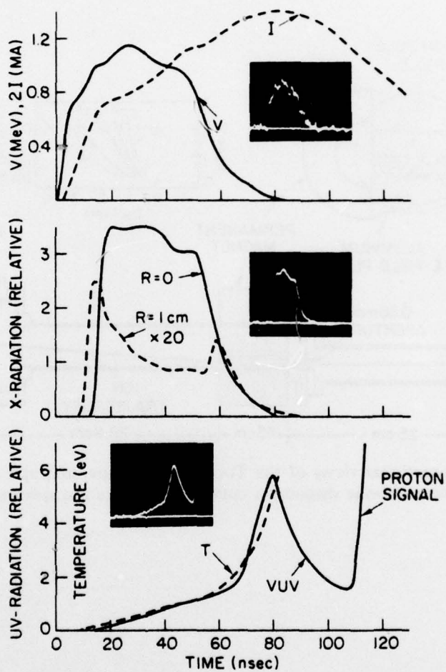
Fig. 3 — (Top) Diode voltage (V) and current (I) from shot 1309. The voltage has been corrected for inductive contribution. (Center) Measured x-radiation signals for shot 1319 from collimated PIN diodes observing a 5 mm diameter area of the anode at r = 0 and 1 cm. (Bottom) Observed signal for shot 1309 from an aluminum XRD filtered by 1/2 \mu\text{m} aluminum which views a 1.2 cm diameter area in the center of the anode. The dashed curve represents a calculated anode surface temperature for the measured electron beam parameters, assuming normally incident electrons, classically absorbed by a 1 cm diameter aluminum target.
