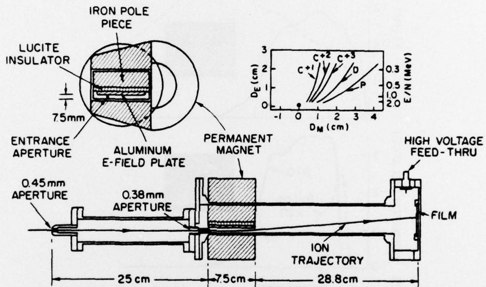
Fig. 2 — Cross-sectional views of the Thomson mass spectrograph and a plot of the parabolic dispersion curves for various ion species
