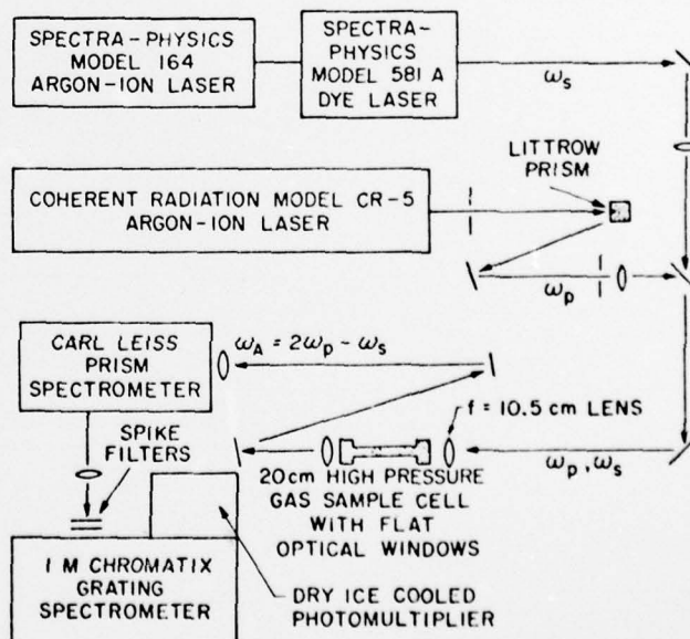
FIG. 1. Experimental layout for coherent anti-Stokes generation in methane gas at 0.4474 \mu\text{m} by collinear mixing of single axial mode lasers, a cw dye laser at 0.6054 \mu\text{m} against an argon ion laser at 0.5145 \mu\text{m} .
