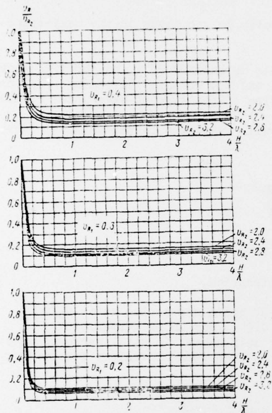
Figure 6. Dispersion of Rayleigh wave velocities v_R in the layer on a half-space. v_{R1} -- the velocity of Rayleigh waves in the layer, km/sec; v_{R2} -- the velocity of Rayleigh waves in the half-space, km/sec.
