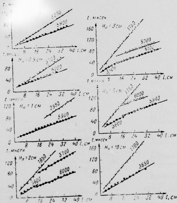
Figure 5. Travel time curves of the principal types of waves during profiling zz on frost, on the surface of a layer (diagram of Figure 1a). \mu - microseconds
