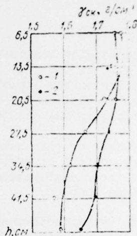
Figure 5. Change of the density of the skeleton with depth in experimental embankments of salinized and unsalinized Langarskiy loess-like loam after eight passes of the FVK-70e compactor. 1 - salinized soil; 2 - unsalinized soil. a - \gamma_{sk}, g/cm^3
