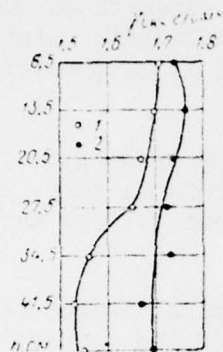
Figure 4. Change of the density of the skeleton with depth in experimental embankments of salinized and unsalinized Langarskiy loess-like loam after four passes of the FVK-70e compactor. 1 - unsalinized soil; 2 - salinized soil r, passes of the FVK-70e compactor, h = 55 cm and W = 16.0\% . a - \gamma_{sk}, g/cm^3
