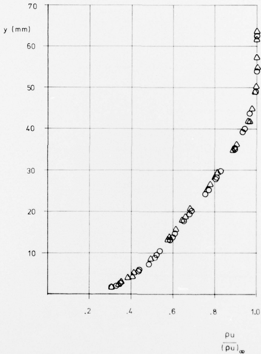
Fig. 14. The normalized mass flow in the boundary layer from measurements with the new mass-flow system and the AVA combined pressure-temperature probe.
