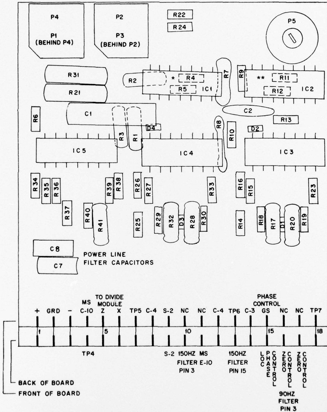
Figure A-11. 90/150 Converter Board.
