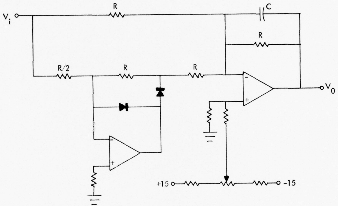
Figure A-4. Absolute Value Circuit.
