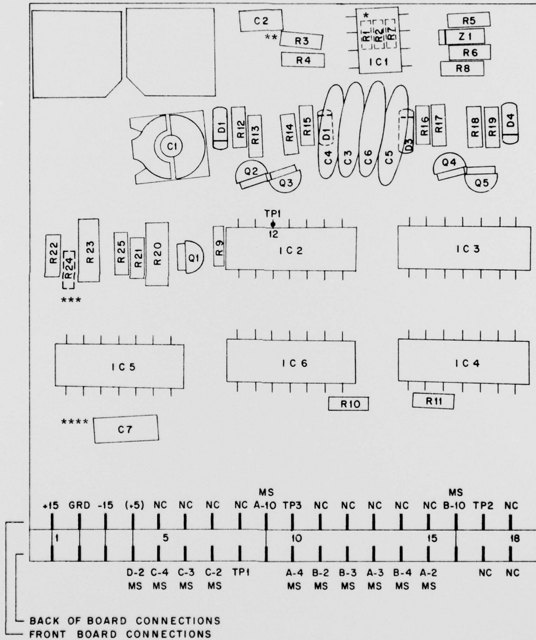
Figure A-12. Calibrator Board.
