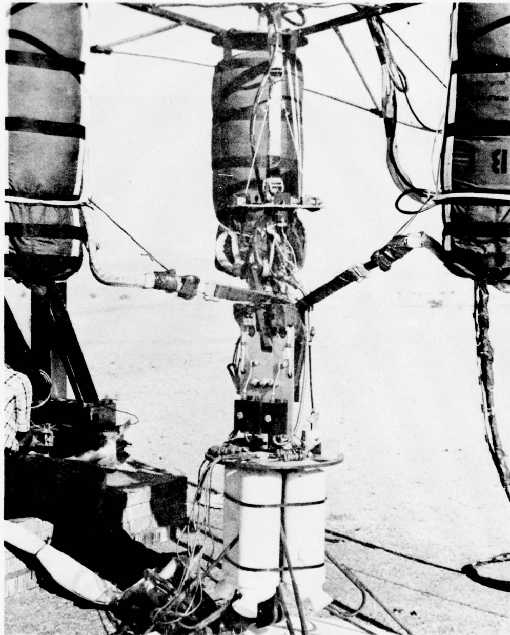
Figure 20. Rocket Cluster/Confluence Fitting
