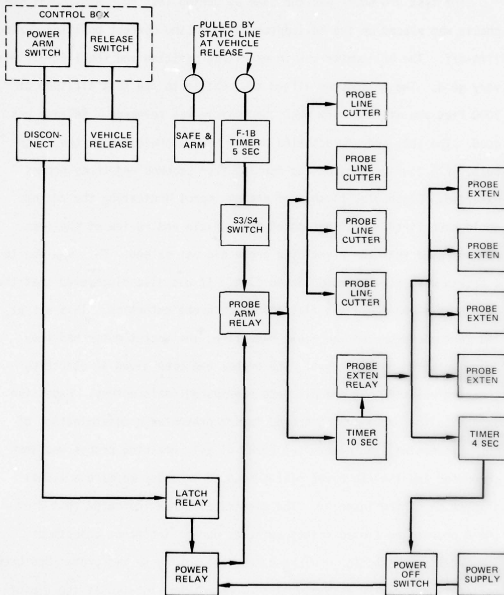
Figure 17. Sequence System - Final Modification
