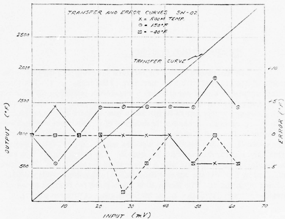
Figure 34 -- Transfer and Error Curves - SN 02
