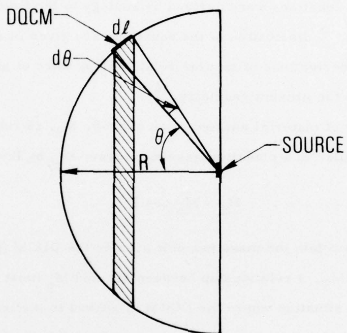
Figure 5. Geometrical considerations for solving relationship of M_T to M_p
