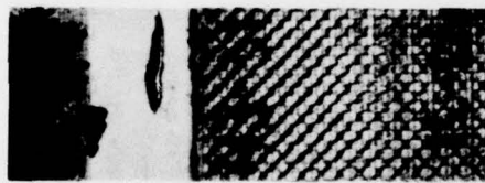
C Interply Failure Nonscrim Side Specimen 43-31
