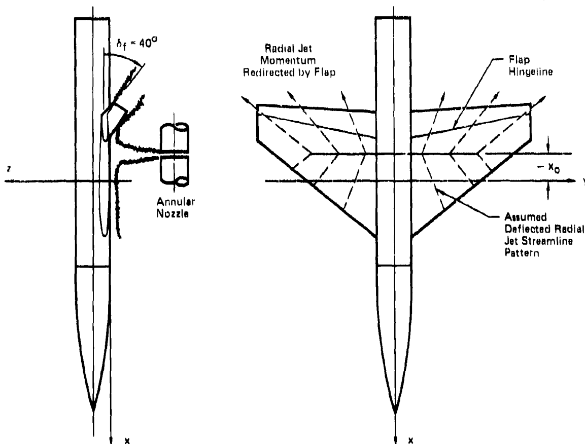
FIGURE 82 CALCULATION OF NORMAL FORCE INCREMENT DUE TO FLAP
