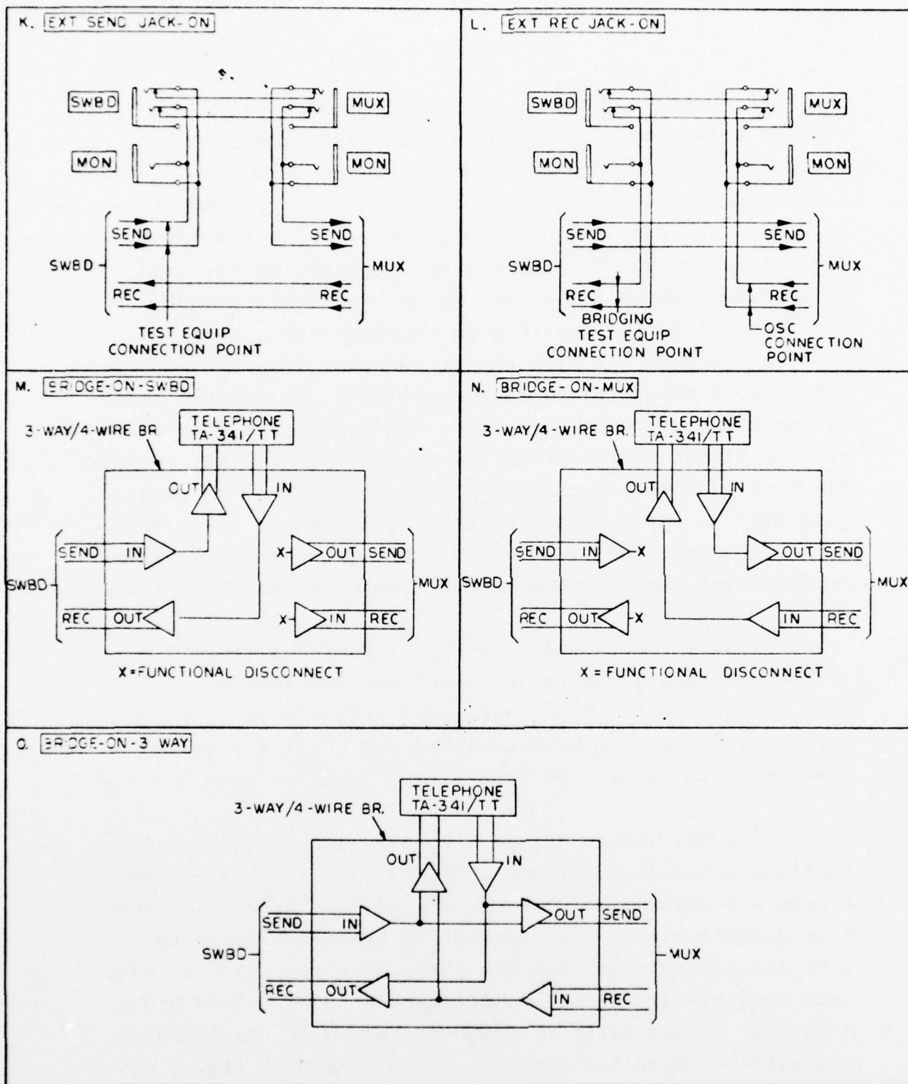
Figure 7. Bridging And Terminating Functions Of Test Select Panel Switches (Sheet 2 of 2)
