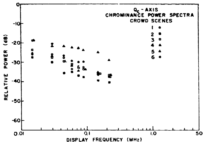
Figure 27. Individual chrominance power spectra for the C_m, Q_c terms of scenes that contain more than ten prominent objects. The numbers next to the symbols in the legend correspond to the scene numbers of Table 9.
