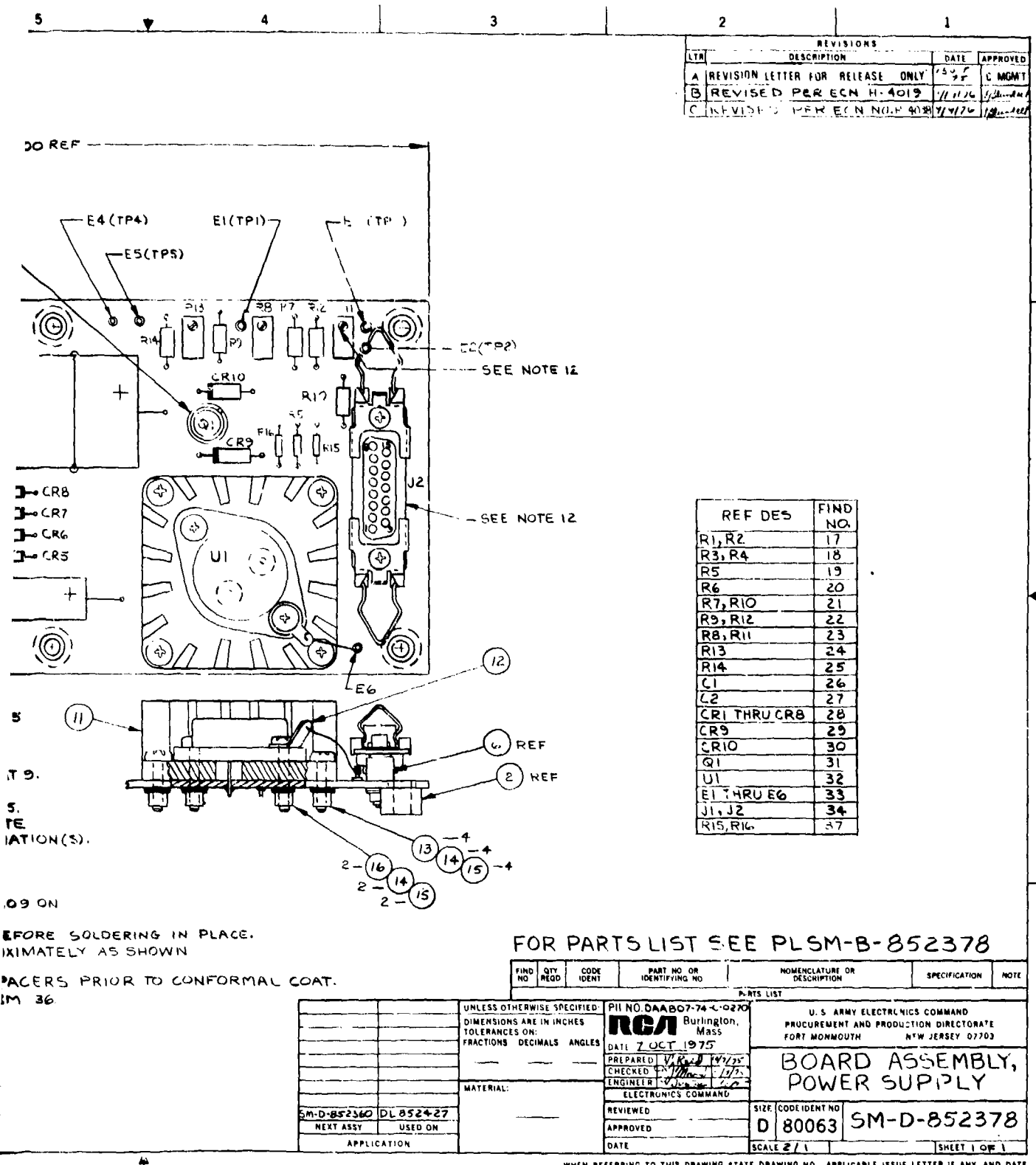
Figure 2-24. STE Power Supply Printed Wiring Board
