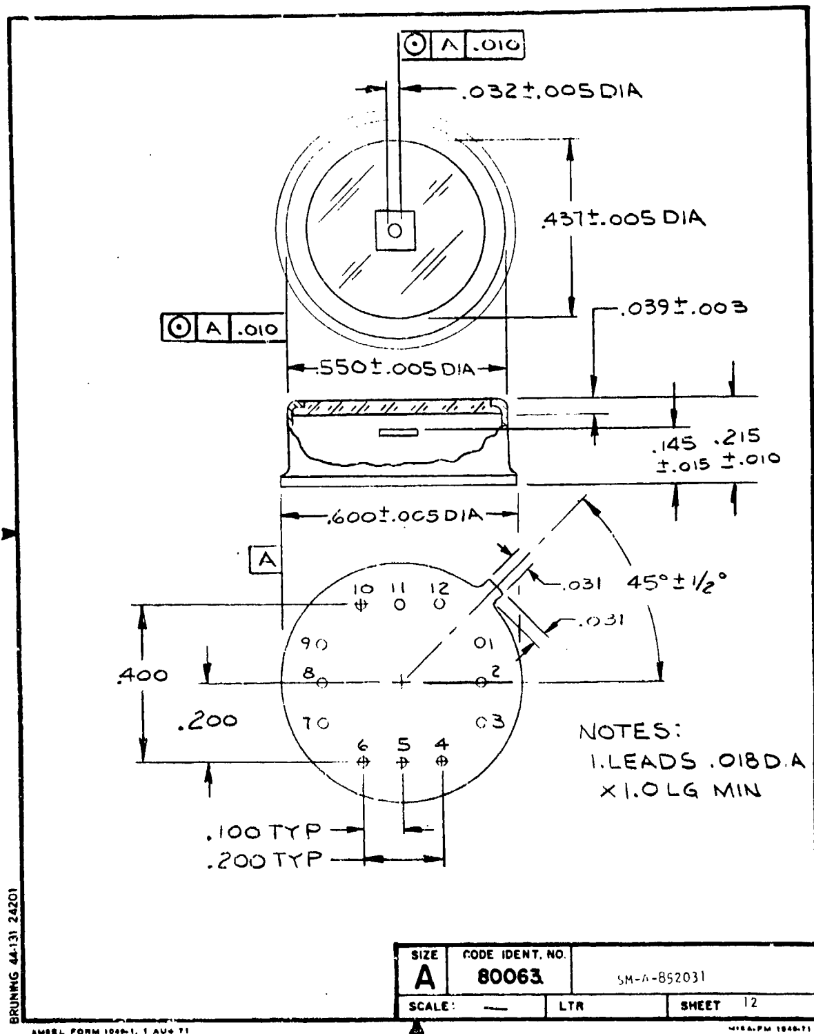
Figure 2-19. Physical Dimensions
