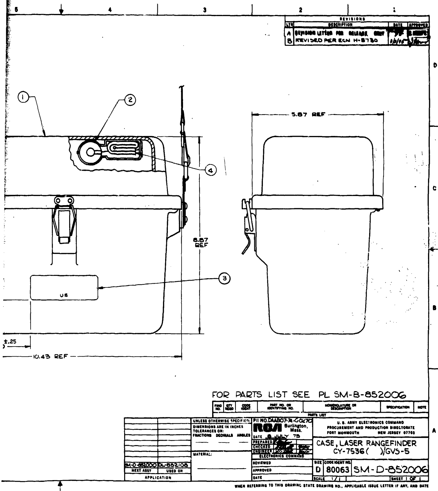
Figure 2-10. Carrying Case
