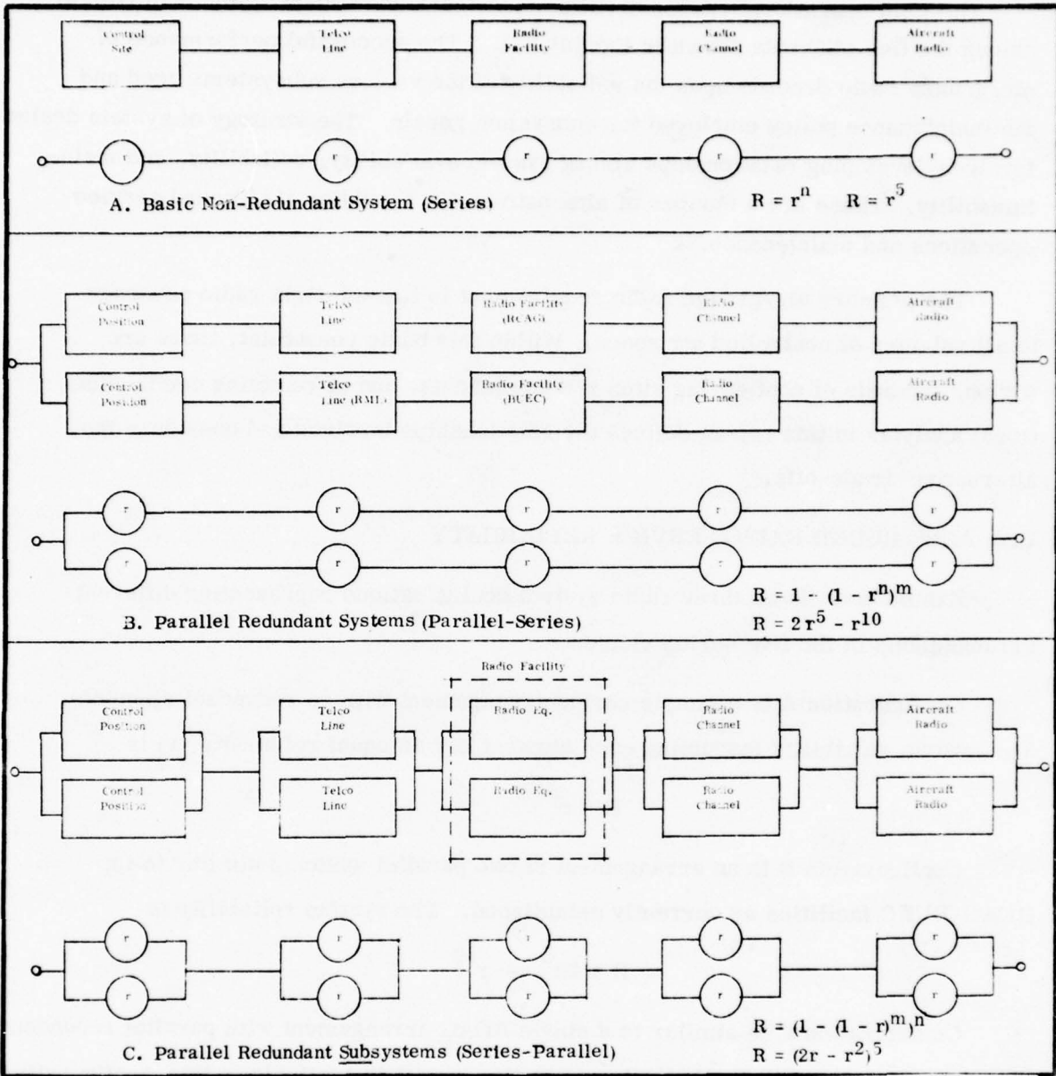
Exhibit 11-2: RELIABILITY FOR REDUNDANT SYSTEMS
